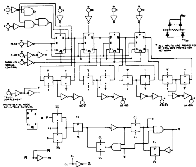
Logic Diagram
