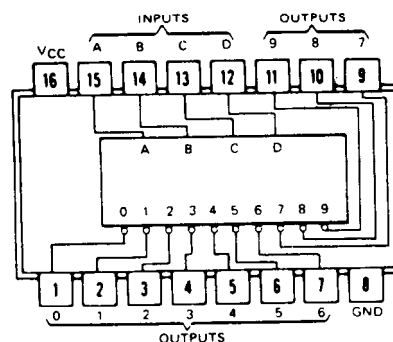
Pin Connection Diagram
