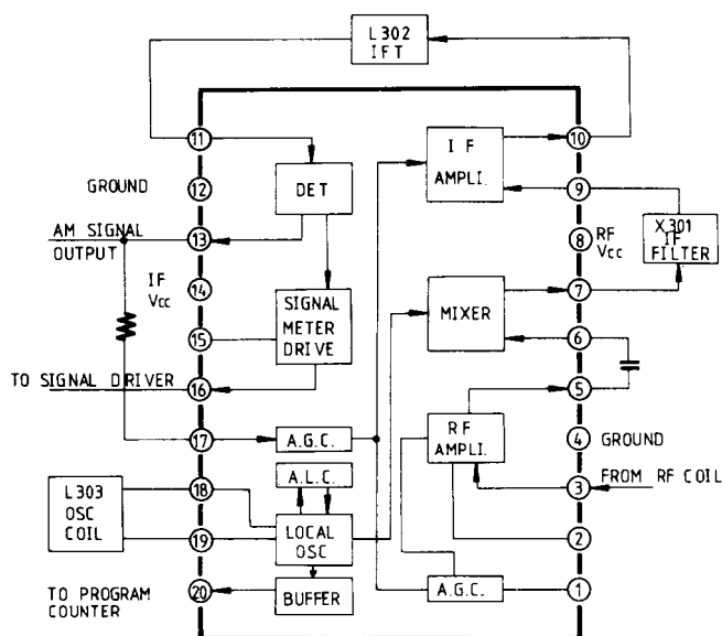
LA1245 (AM radio system)
