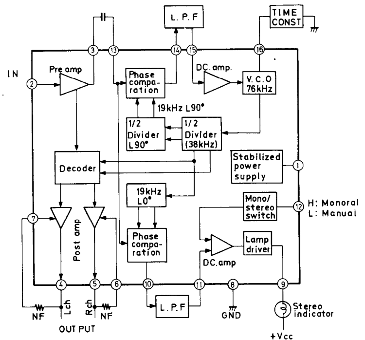
HA12016 (Stereo decoder)
