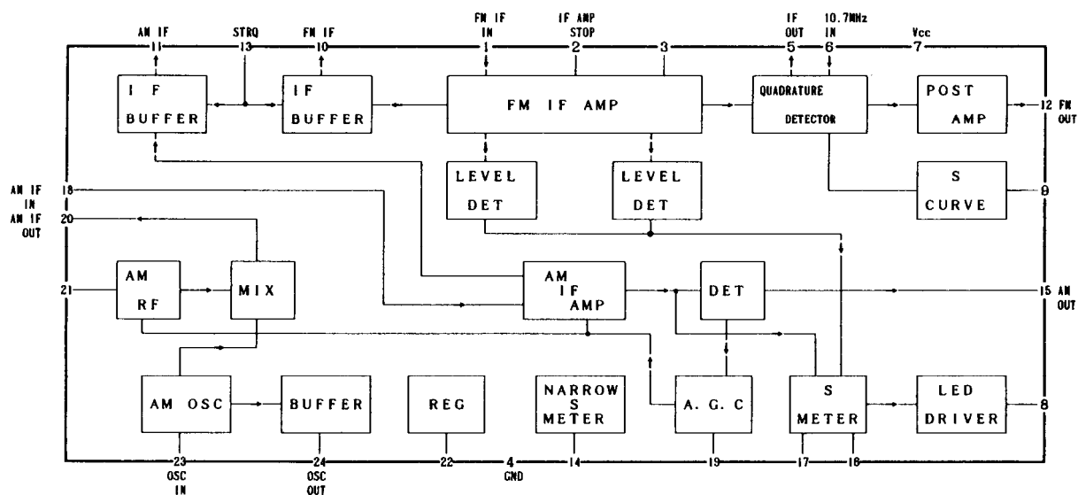
LA1266 (FM IF/AM radio system)
