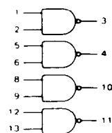
LOGIC DIAGRAM
