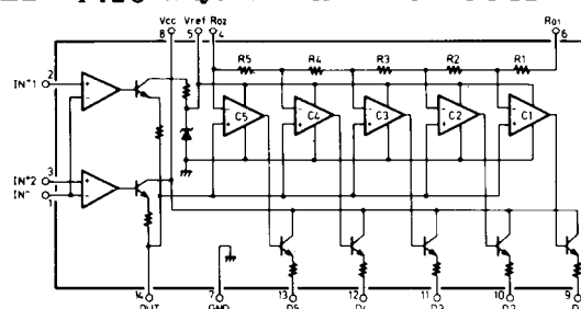
LB-1426 EQUIVALENT CIRCUIT
