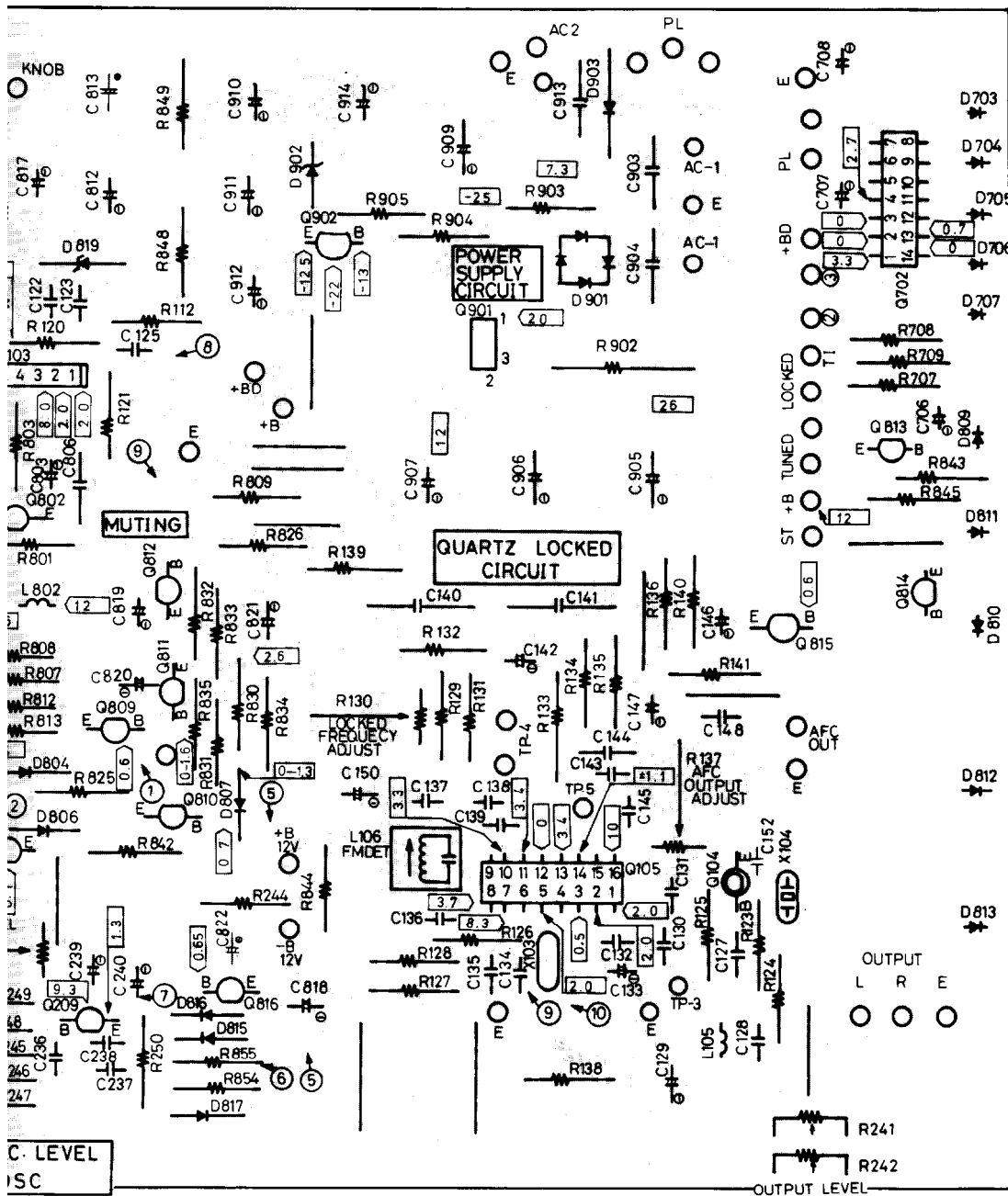
BA-402 EQUIVALENT CIRCUIT
