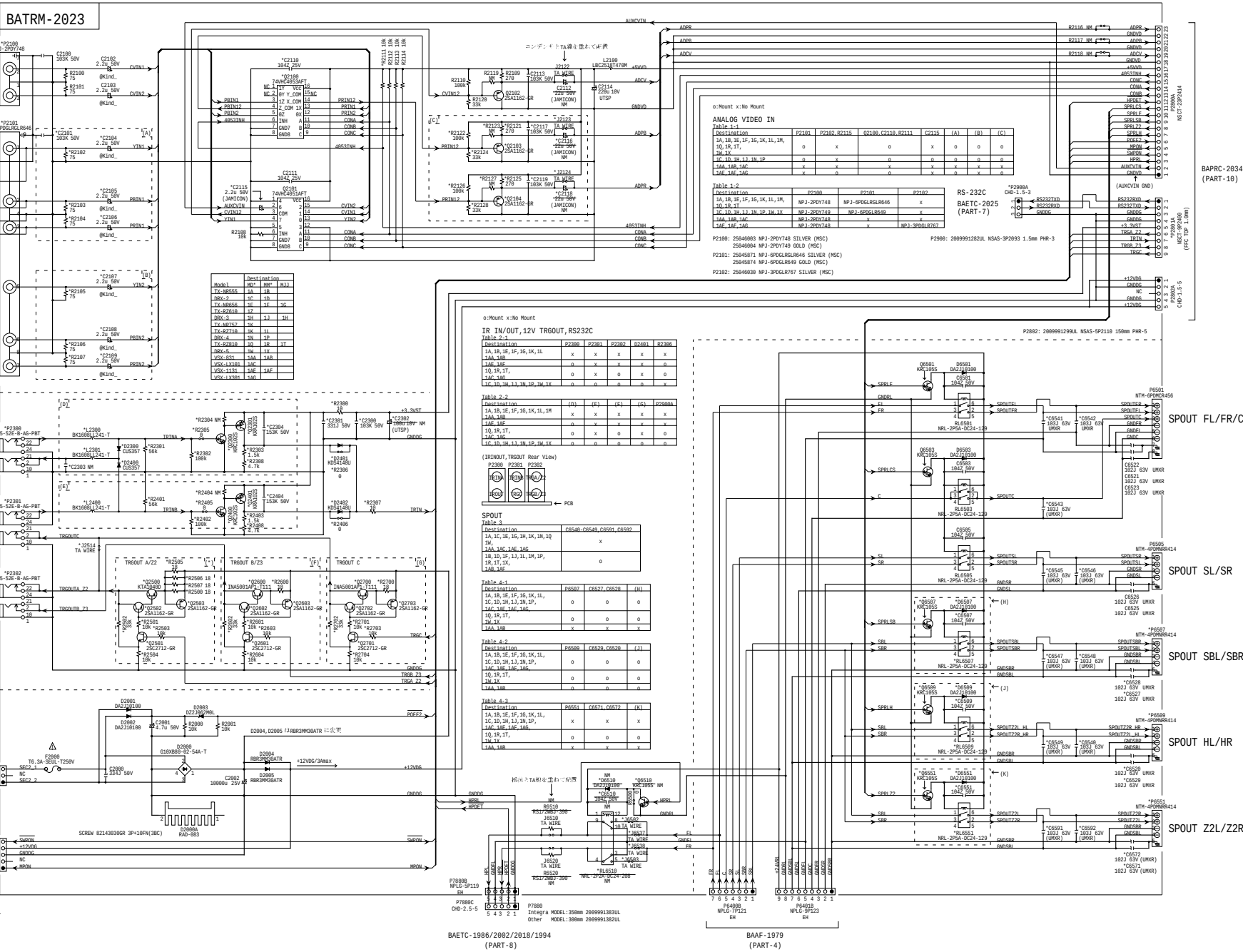
MODEL NO. TX-NR555/656/757, TX-RZ610/710/810, HT-R695, DRX-2/3/4/5 SCHEMATIC DIAGRAM(PART-7) VIDEO, SPOUT, IR/12VTRG SECTION
