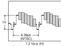
Component Y waveform
