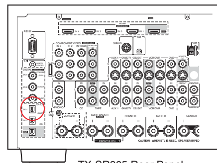
TX-SR805 Rear Panel (Refer to Page 2 for TX-SR705)
