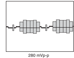
Component PR waveform
