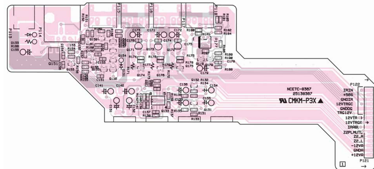
U3 Control terminal PC board (NAETC-8367)
