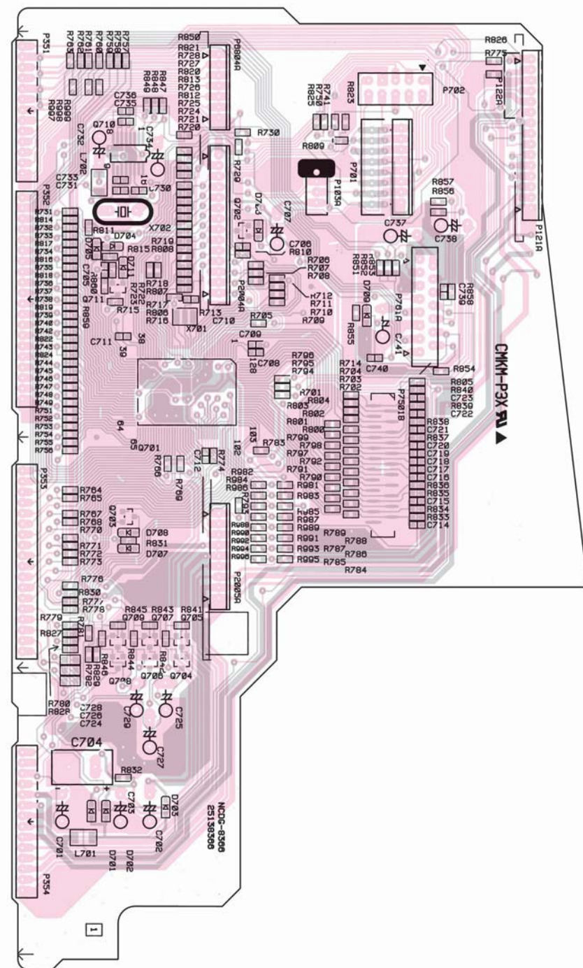
U2 NADG-8366 Main connector PC board
