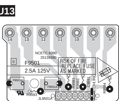
Fuse terminal PC board (NAETC-8390)
