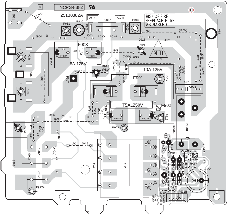
U5 Primary circuit PC board (NAPS-8382)
