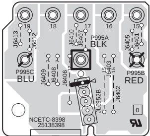
U17 Secondary circuit PC board (NAETC-8398)
