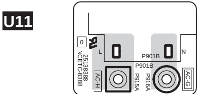
AC inlet terminal PC board (NAETC-8388)
