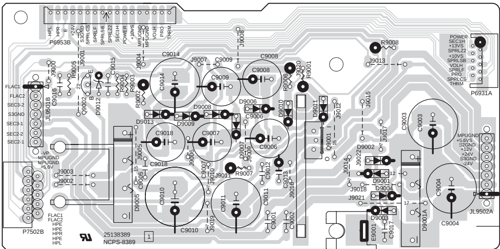
U12 Secondary circuit PC board (NAPS-8389)
