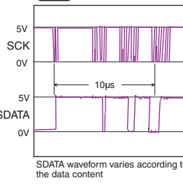
SCK/SDATA waveform (WF61) SD-13:D2, F2
