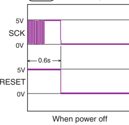
SCK/RESET waveform (WF63) SD-13:D2, F2
