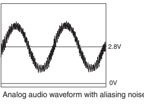
(WF09) DAC_OUT- (SD-9:E4)
