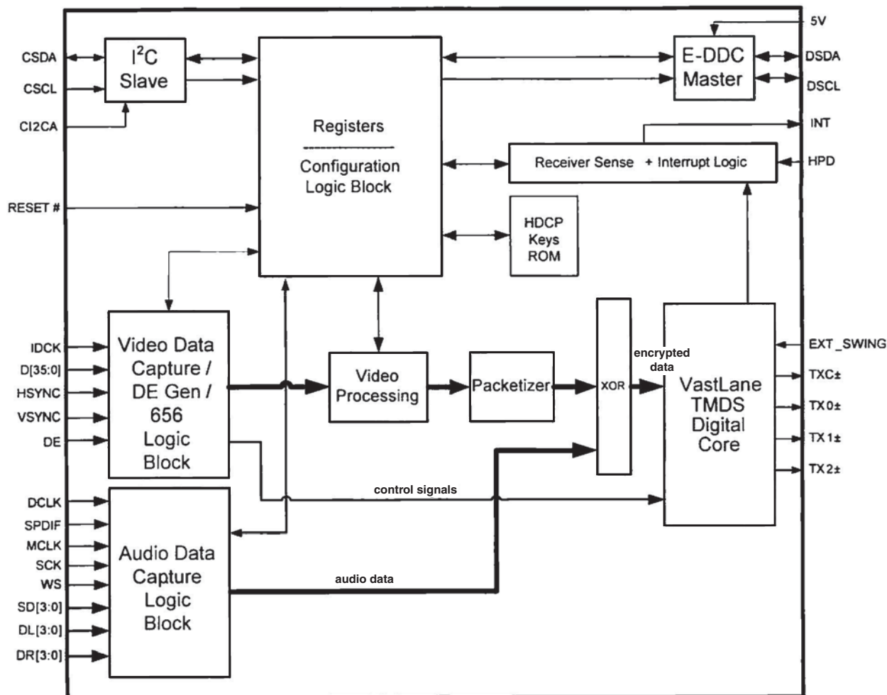
BLOCK DIAGRAM
