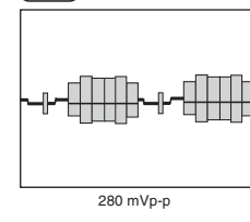
S-Video C waveform (WF23) SD-6:B5
