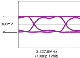
HDMI D0,D1,D2 waveform (WF41) SD-17:B5/SD-18:4G
