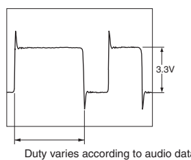
(WF03) SAI_SDOUT (SD-9:B4)
