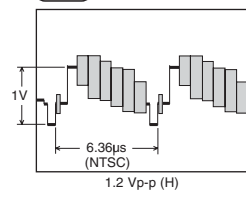
Composite waveform (WF21) SD-6:B5
