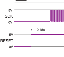
SCK/RESET waveform (WF63) SD-13:D2, F2
