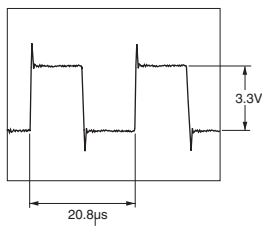
(WF06) CX_SDIN1 (SD-9:D4)
