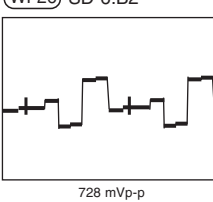
Component PR waveform (WF26) SD-6:B2
