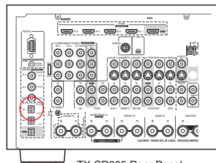
TX-SR805 Rear Panel (Refer to Page 2 for TX-SR875)
