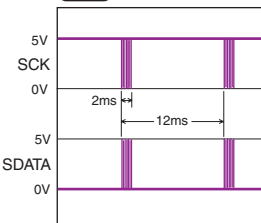
SCK/SDATA waveform (WF61) SD-13:D2, F2
