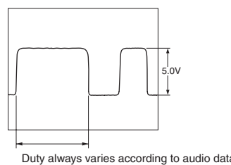
(WF02) COAX1 (SD-9:C2)
