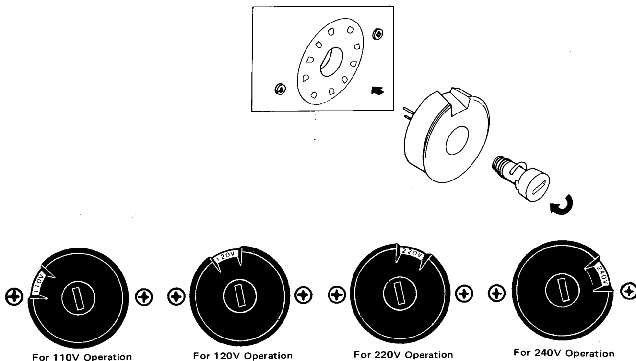
Figure 2. Voltage Conversion Chart
