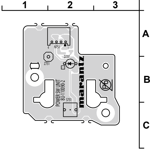
POWER SW (COMPONENT SIDE)
