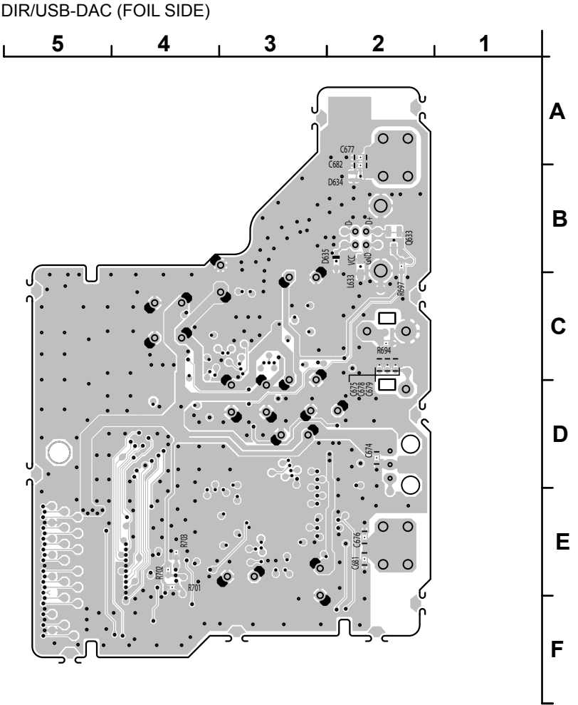
DIR/USB-DAC (FOIL SIDE)
