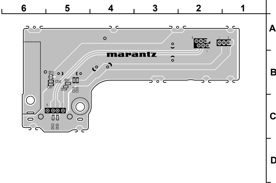
FRONT USB (FOIL SIDE)
