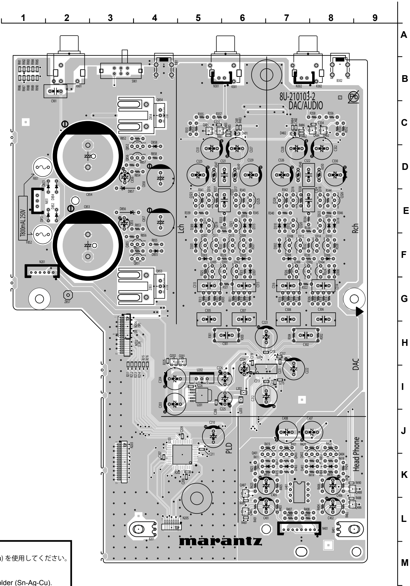
DAC/AUDIO (COMPONENT SIDE)
