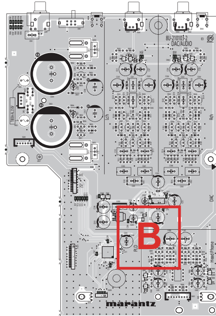
DAC/AUDIO UNIT (component side)
