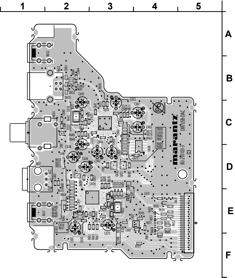
DIR/USB-DAC (COMPONENT SIDE)
