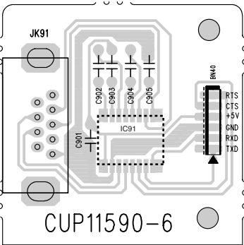
RS232C [SR6400 only] IC91
