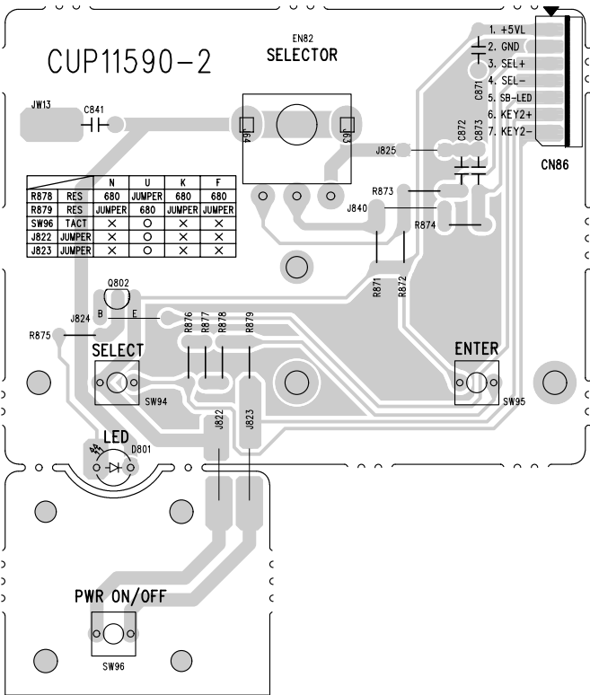
ENCODER & TACT Q802
