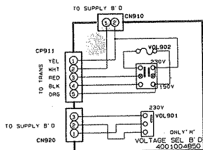
VOLTAGE SELECTOR BOARD (PCB14) -CIRCUIT DIAGRAM
