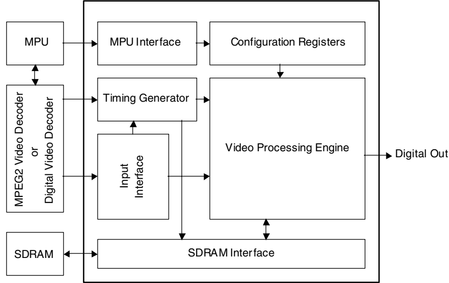
Fig. 2-1: System Block Diagram
