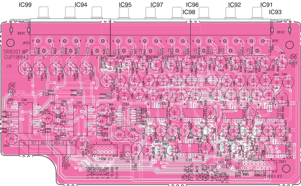
COMPONENT PWB A (SR8001 only)
