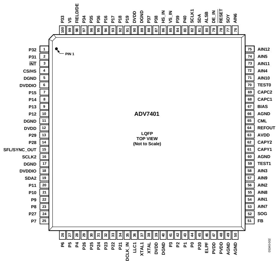
Figure 2.ADV7401 Pin Configuration
