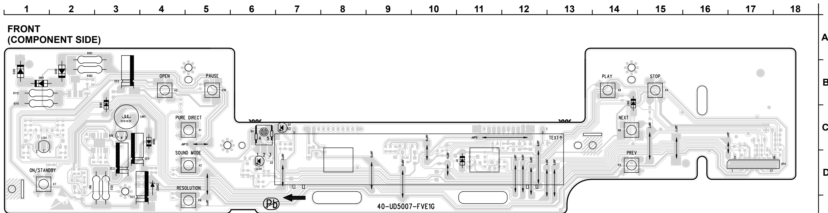
PWD1G (COMPONENT SIDE)
