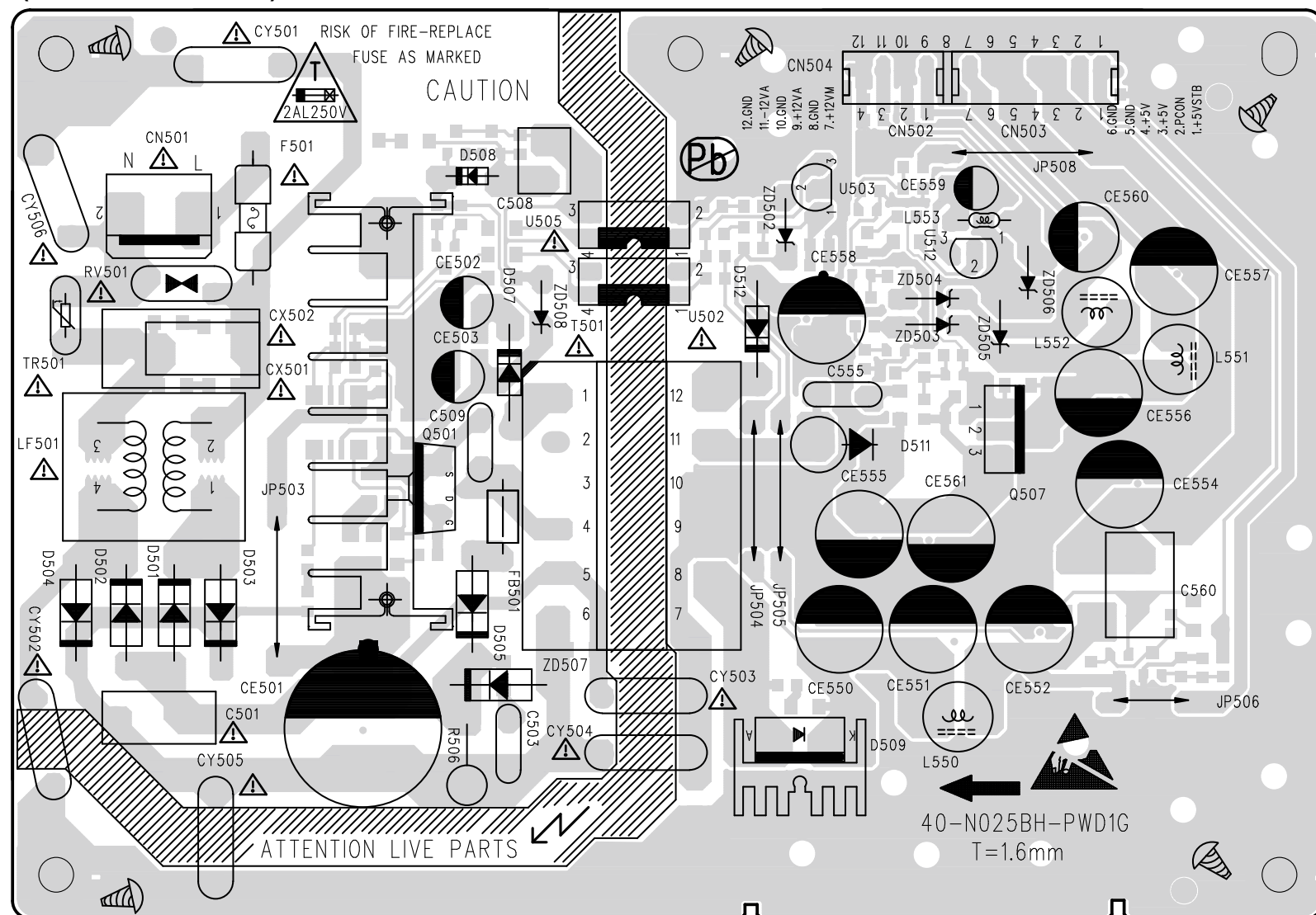
PWD1G (COMPONENT SIDE)
