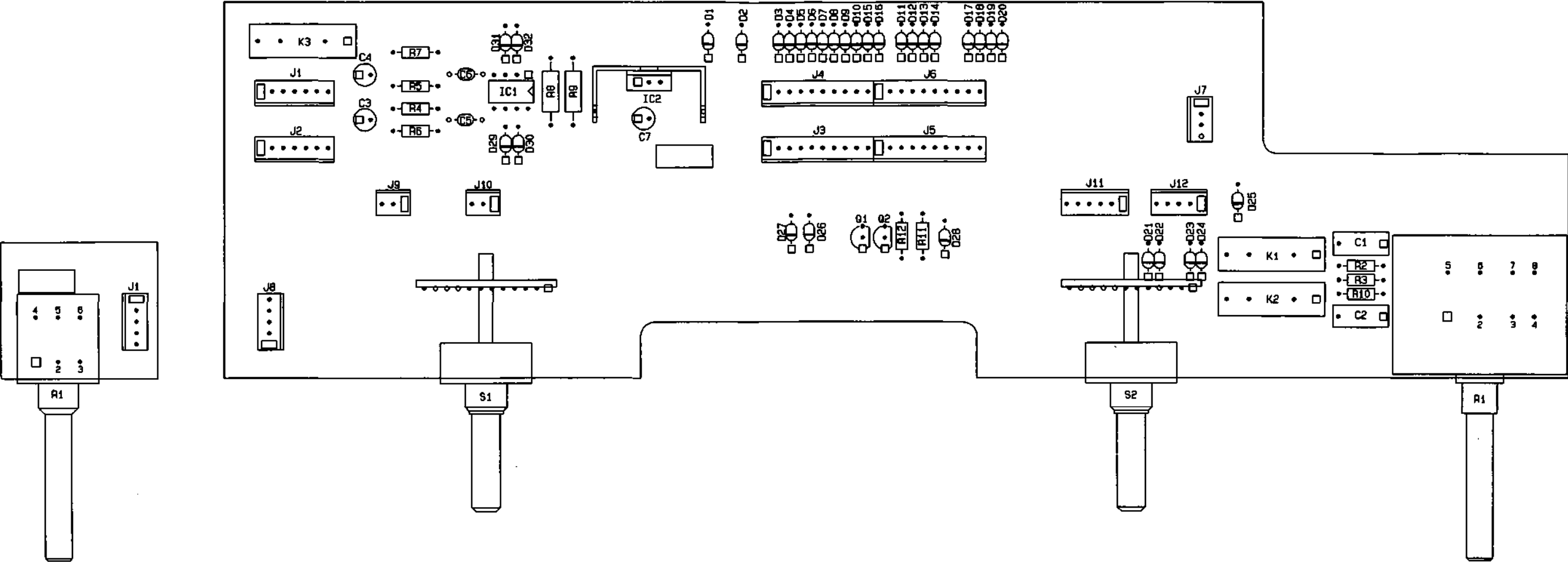
CONTROL PCB 048479
