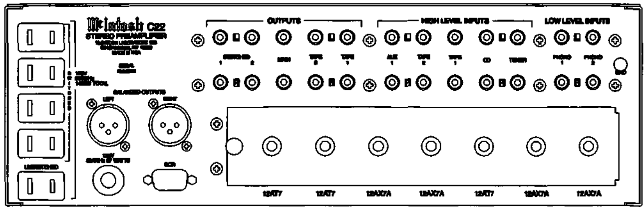
Fig. 1 Rear view
