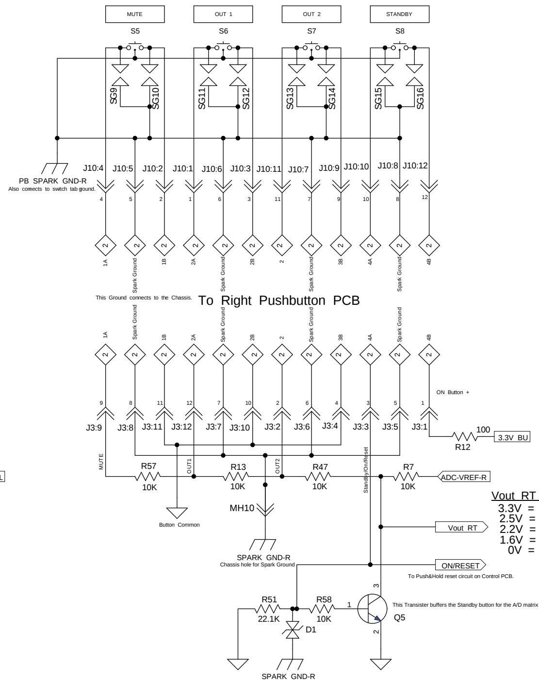
Right Pushbutton PCB
