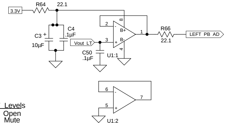
Left Pushbutton A/D Buffer
