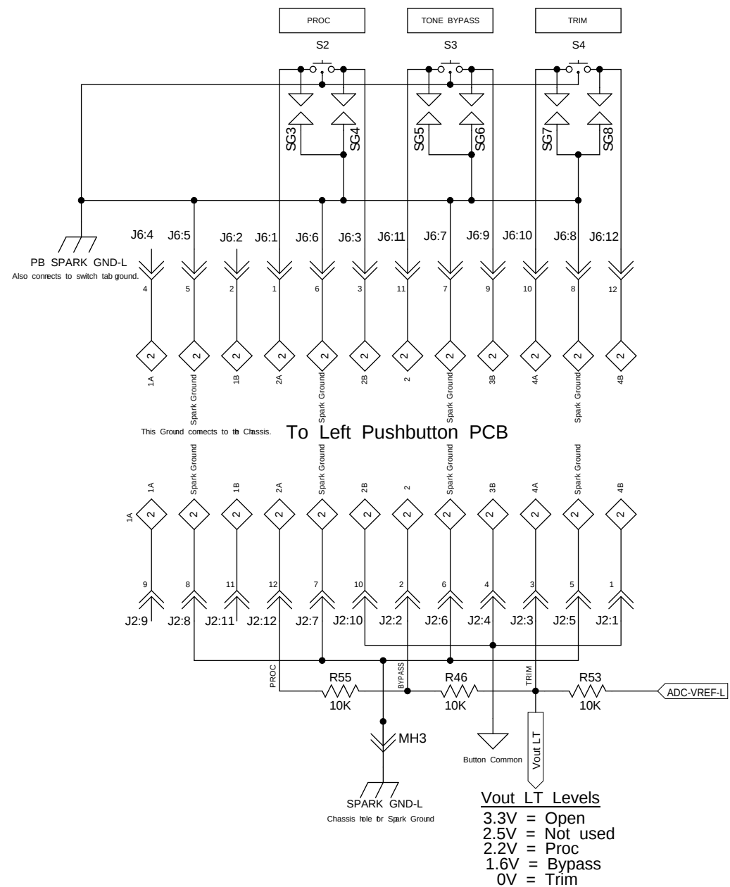
Left Pushbutton PCB
