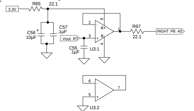
Right Pushbutton A/D Buffer
