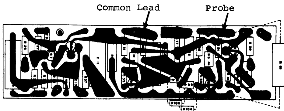
POWER OUTPUT PRINTED CIRCUIT BOARD
