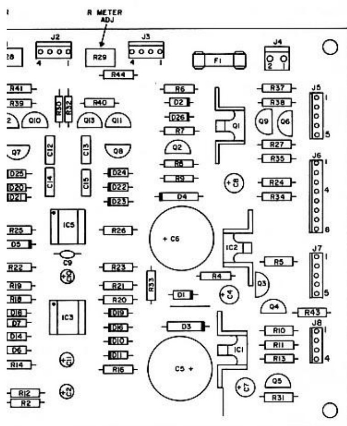
METER/REGULATOR PCB 048496
