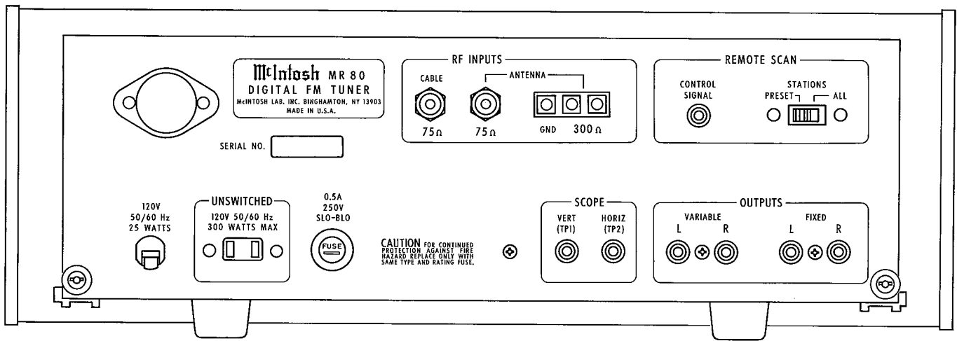
Fig. 0-3. REAR VIEW
