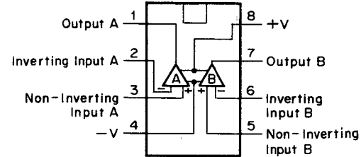
Fig. 13.5 Operational Amp. IC
