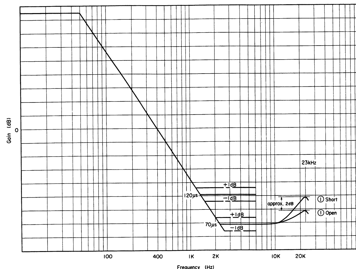
Fig. 6.20 Playback Equalization Curve (1-7/8 ips)
