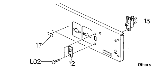
8.17. Rear Panel Ass'y (D08)
