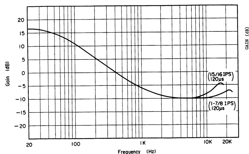
Fig. 6.21 Typical Playback Equalization Curve (1-7/8 / 15/16 ips)
