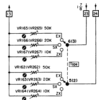
Fig. 6.11 14. Record Head Height and Azimuth
