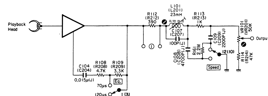
Fig. 6.19 Playback Amp.
