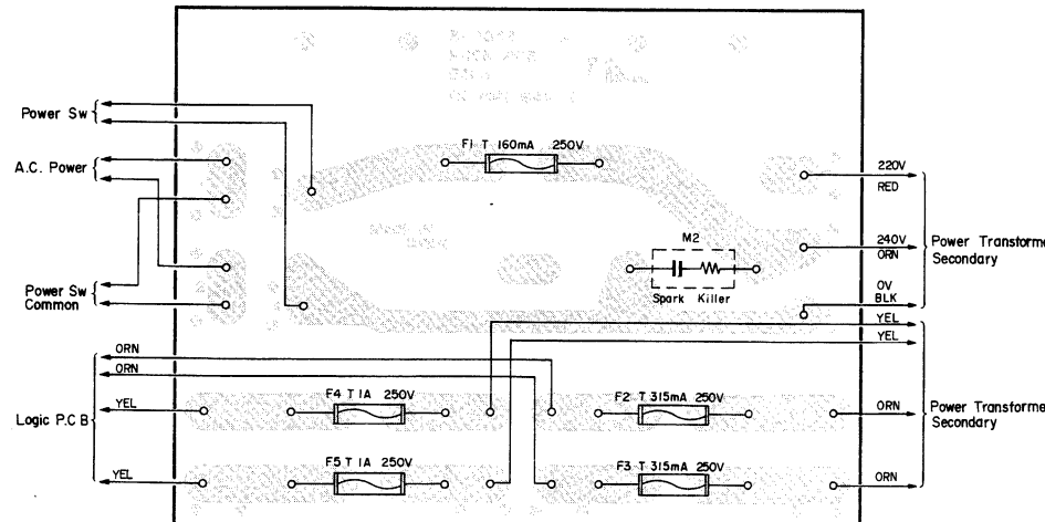
Fig. 7.6.3 UK & Australia
