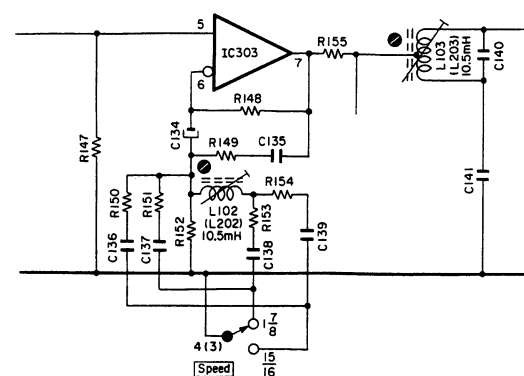
Fig. 6.7 11. Record Amp. Equalizer 12. Bias Trap (Record Amp.)
