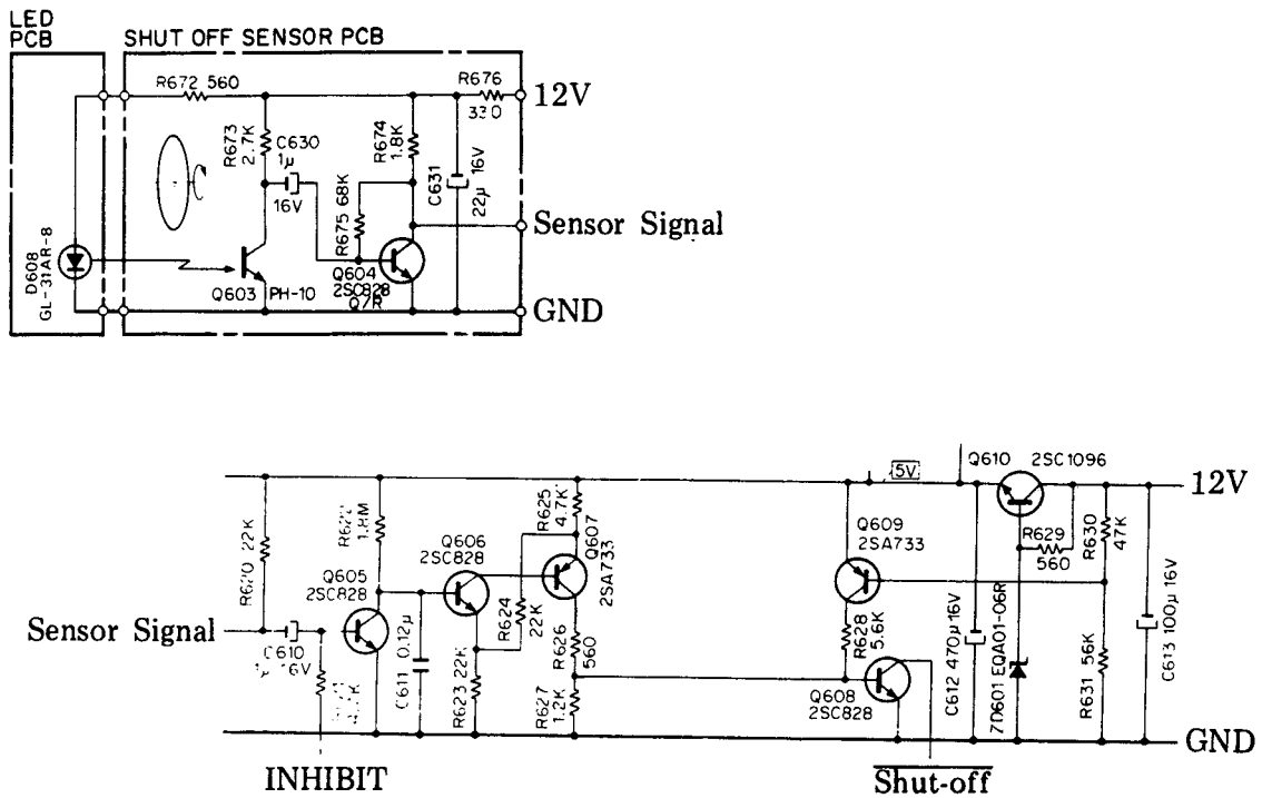
Fig. 2.26 Shut-off Sensor and Detector Circuit Diagram
