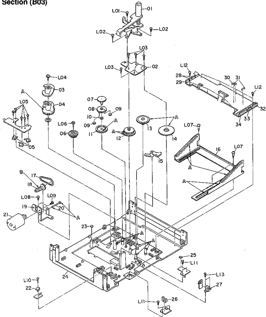
7.5. Main Chassis Section (B03)
