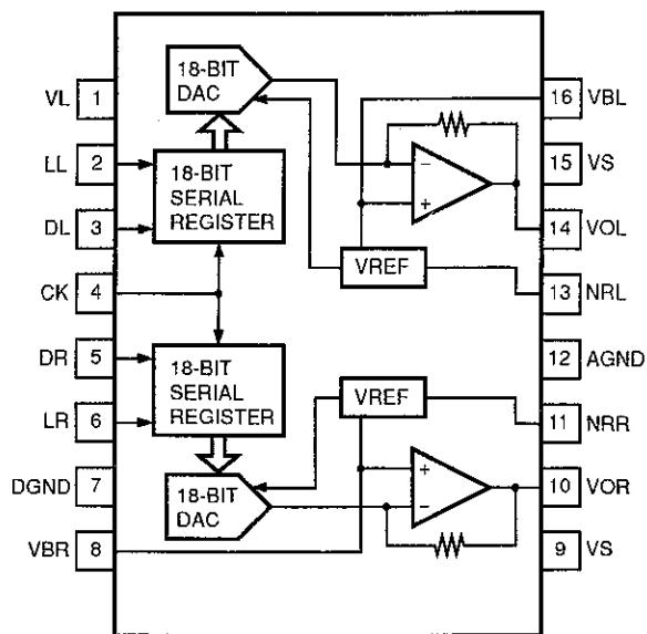
Fig. 9.6 Digital-to-Analog Converter AD1868R (MB-9)
