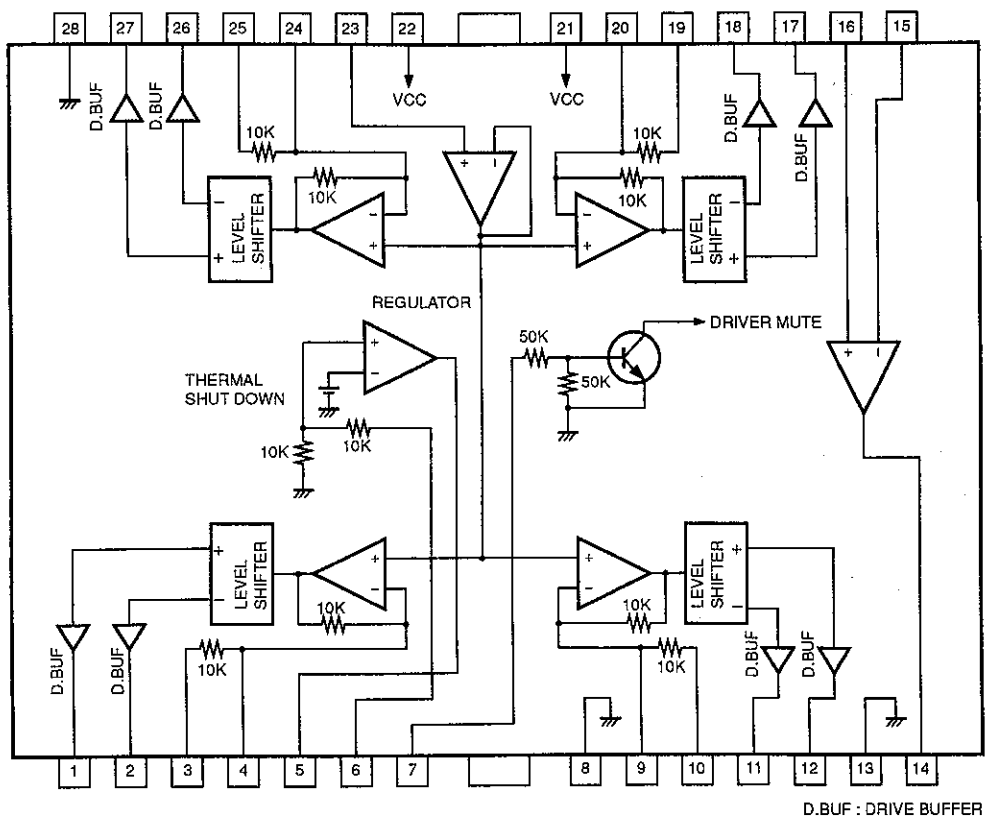
Fig. 9.8 Driver BA6296FP
