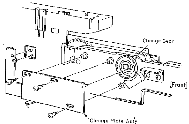
Fig. 3.1.2 Positioning of the Change Gear
