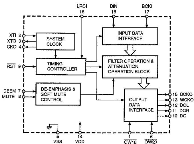
Fig. 9.5 8-Times Oversampling Digital Filter SM5841CS (MB-9)
