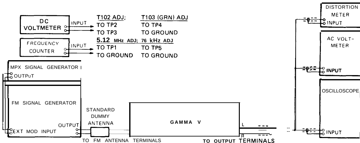
Figure 6. Test Equipment Hook-up
