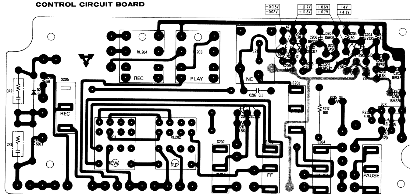
CONTROL CIRCUIT BOARD
