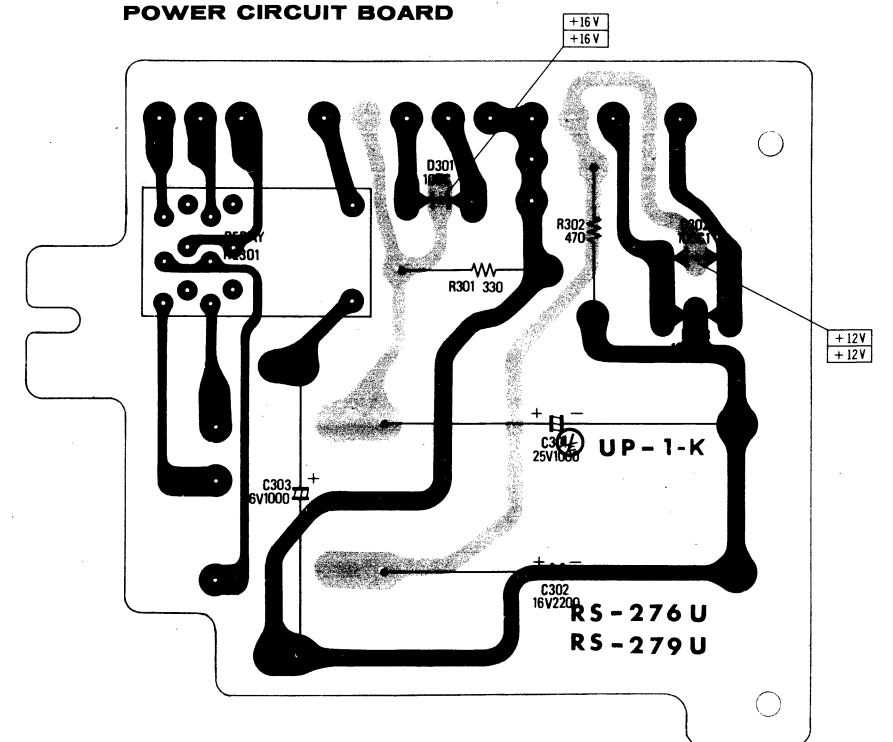
POWER CIRCUIT BOARD
