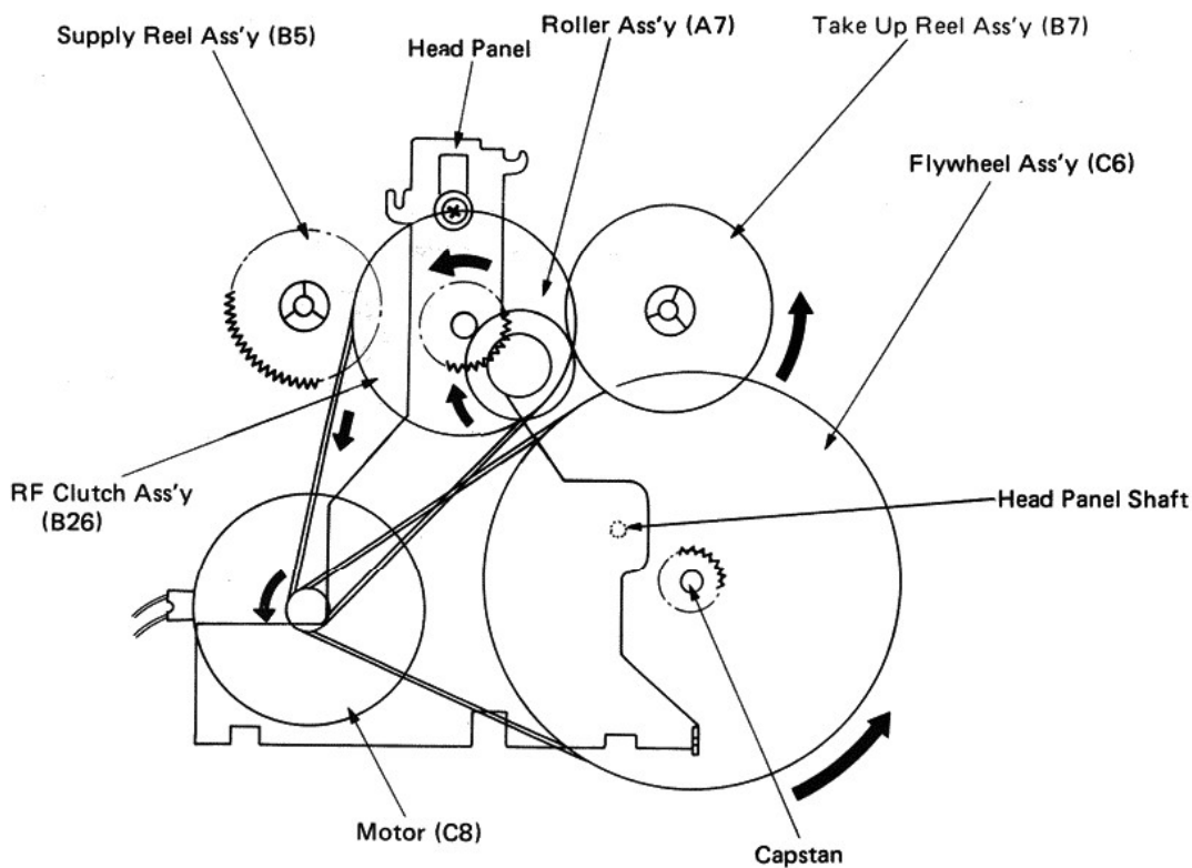
Fig. 5 Front View
