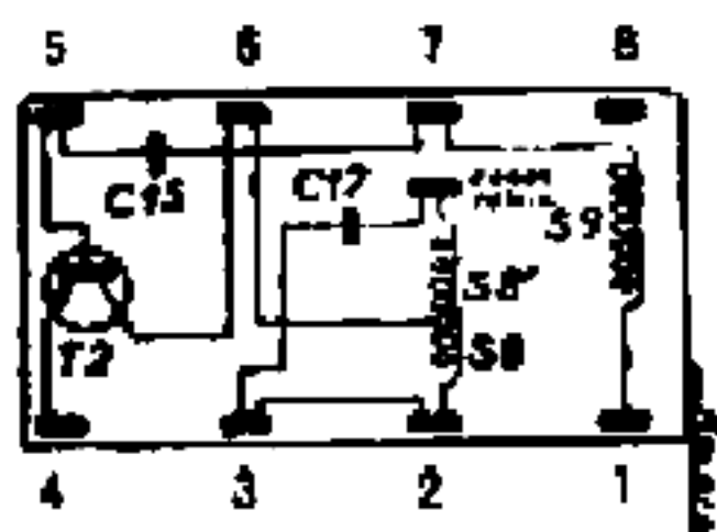
Filter F.1.2
