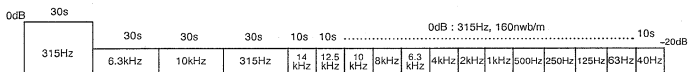
Fig. 7-3 Constants of the test tape STD-331B
