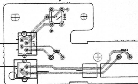
LED assembly
