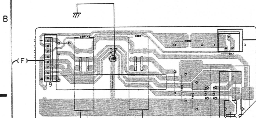
HEADPHONE assembly
