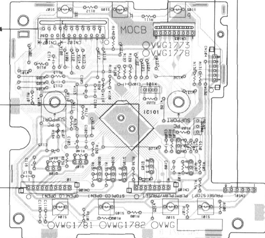
MOCB ASSY
