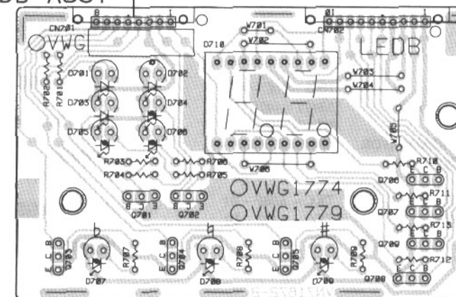
LEDB ASSY
