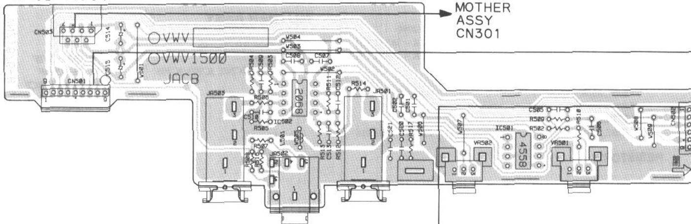
JACB ASSY
