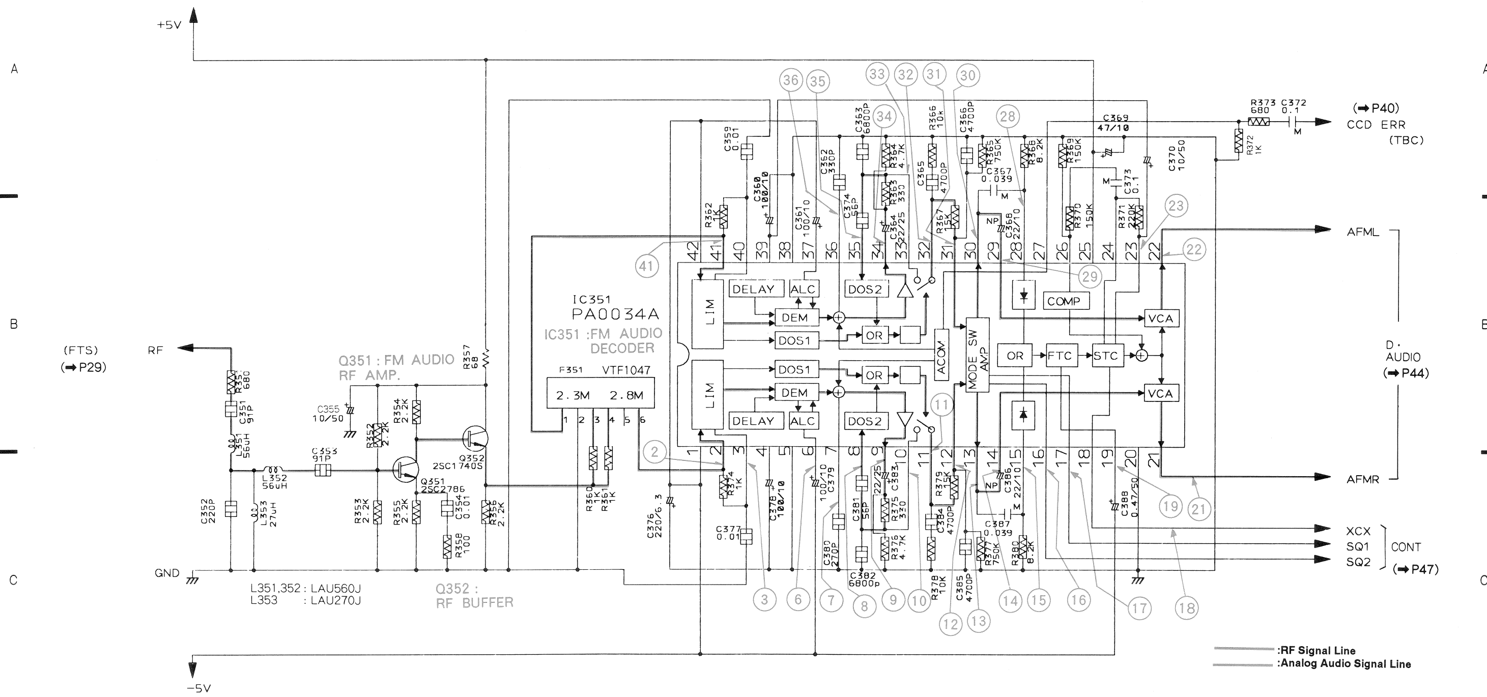
● IC351 (PA0034A)
