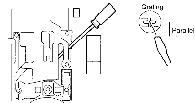
(Top view) Screwdriver inserting direction
