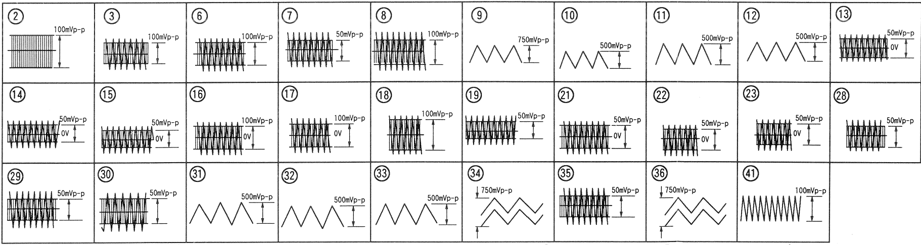
● IC351 (PA0034A)
