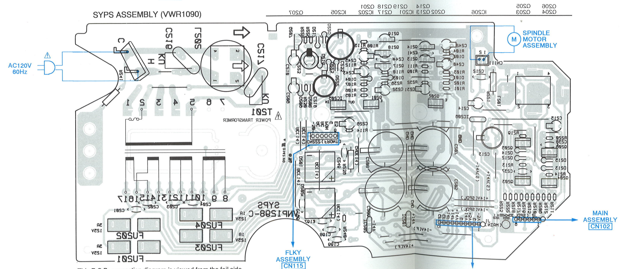
This P.C.B. connection diagram is viewed from the foil side.
