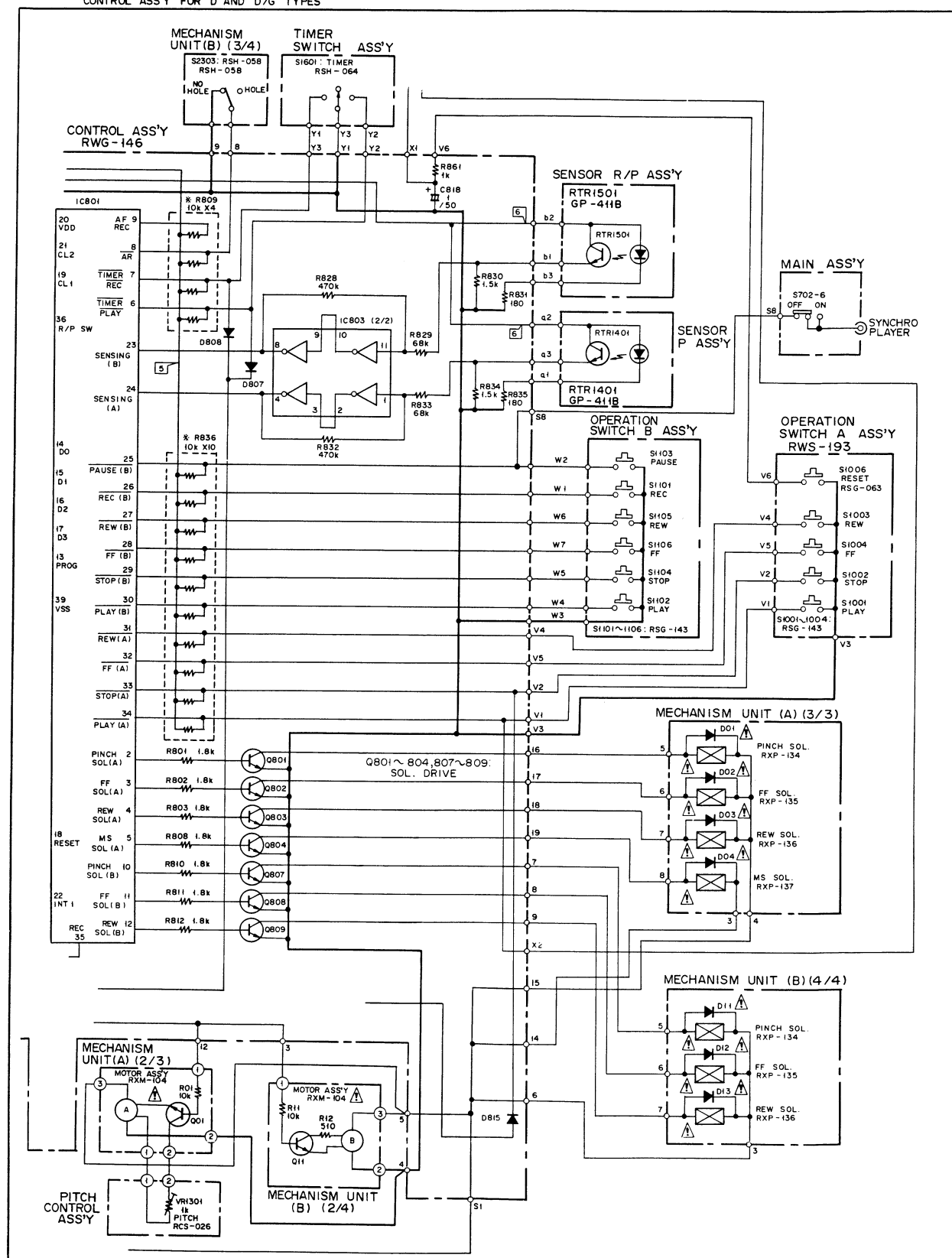
CONTROL ASSY FOR D AND D/G TYPES
