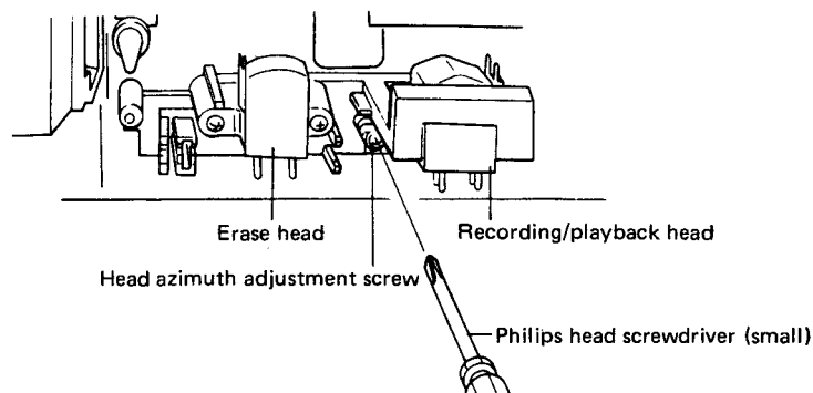
Fig. 10-3 Head azimuth adjustment
