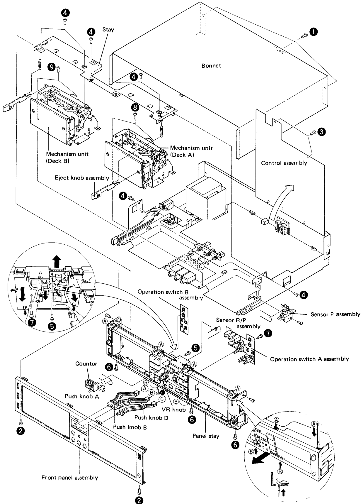
Fig. 3-1 Disassembly
