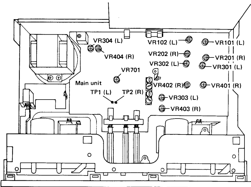
Fig. 10-2 Adjustment locations
