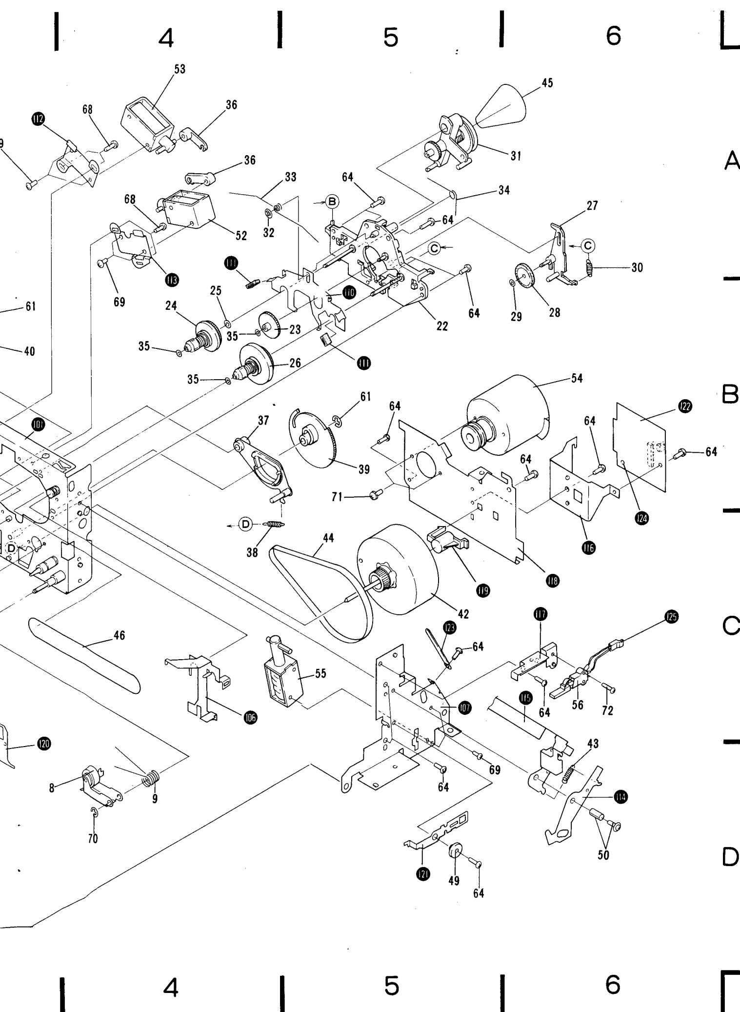
Parts list of Mechanism unit (Deck A)
