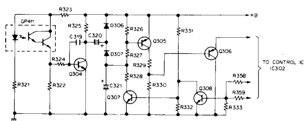
Fig. 6-4 Auto-stop circuit
