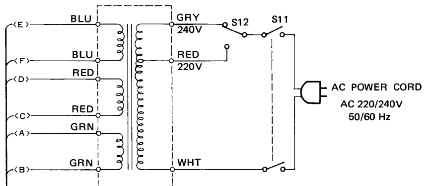
T1 POWER TRANSFORMER
