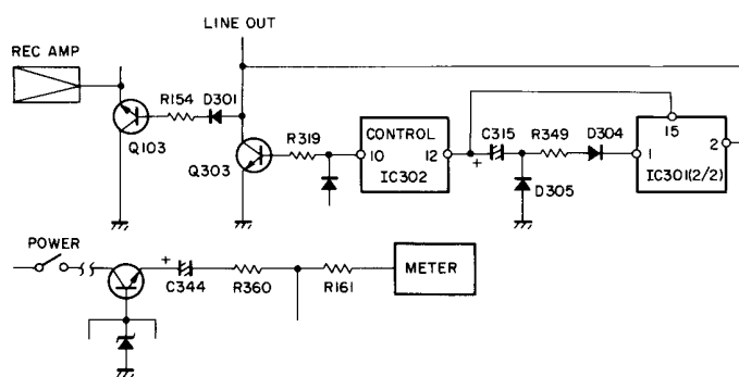
Fig. 6-5 Muting circuit
