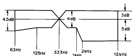
Fig. 8-4 Frequency response
