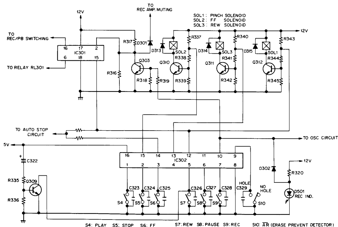
Fig. 6-1 Control circuit
