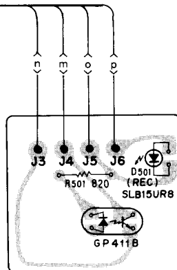
SENSOR Ass'y RWX-402
