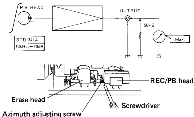
Fig. 8-2 Head azimuth adjustment
