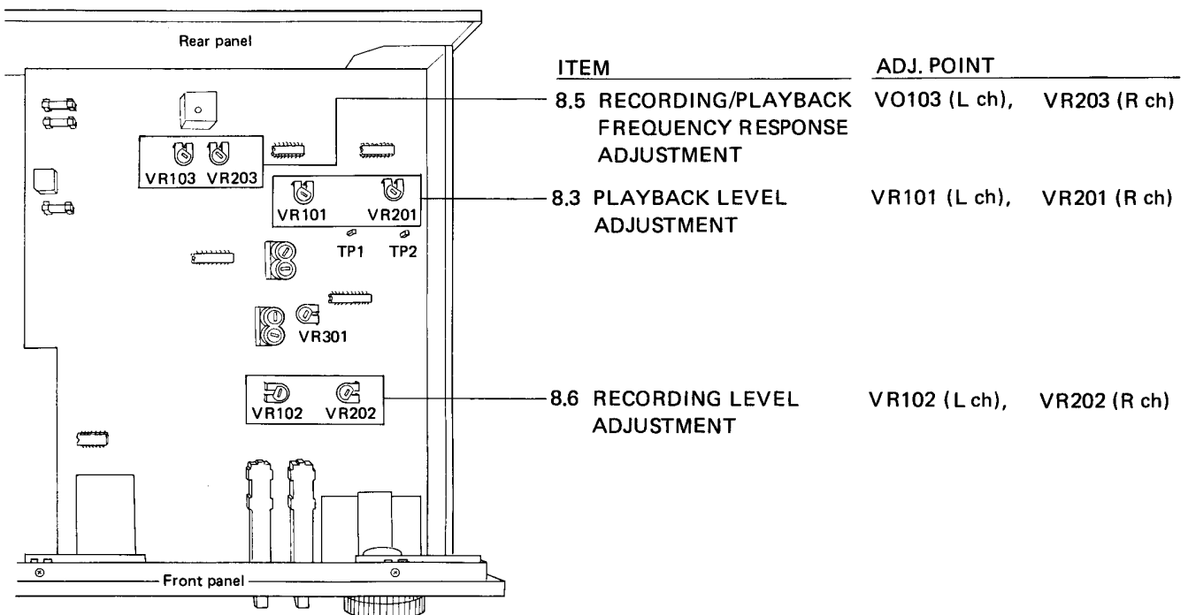
Fig. 8-3 Adjustment points
