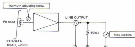
Fig. 13-4 Head azimuth adjustment
