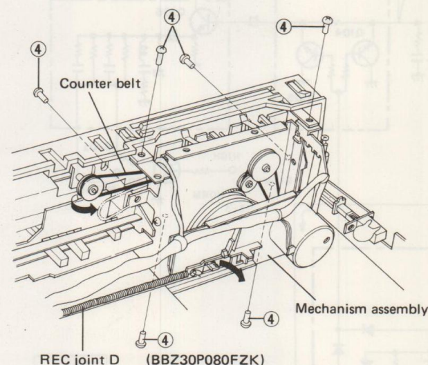
Fig. 3-2 Disassembly 2
