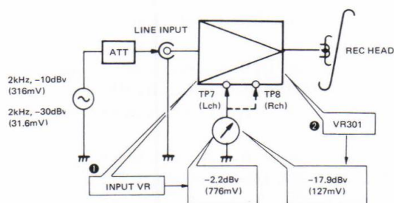
Fig. 13-3 Dolby NR adjustment
