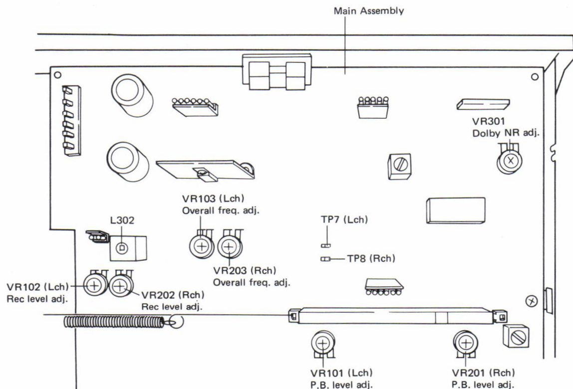
Fig. 13-2 Adjustment points
