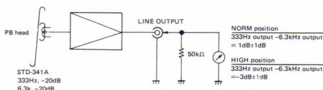
Fig. 13-5 Playback equalizer check
