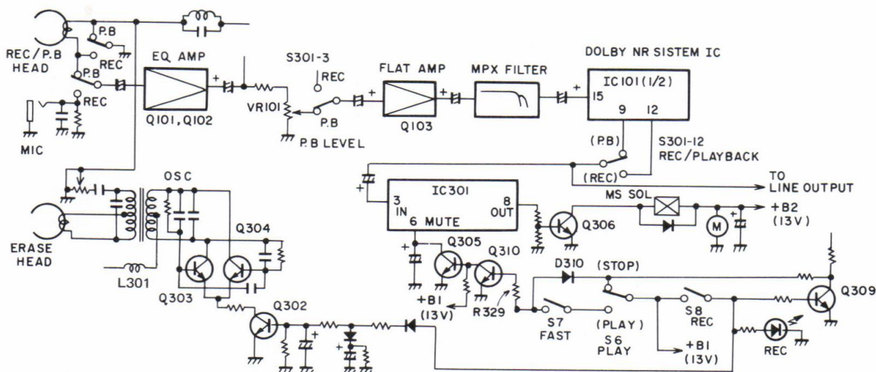
Fig. 6-2 MS operation
