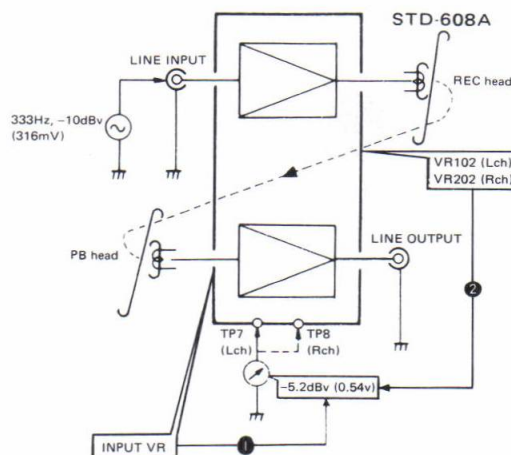
Fig. 13-9 Recording level adjustment
