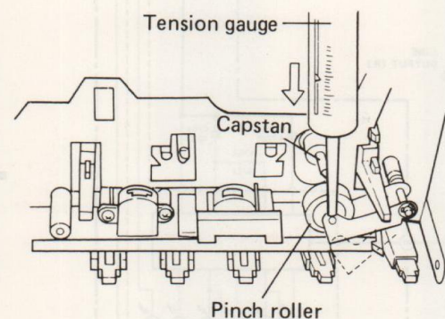
Fig. 12-1 Pinch roller pressure adjustment
