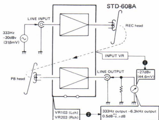
Fig. 13-8 Recording/Playback frequency response adjustment
