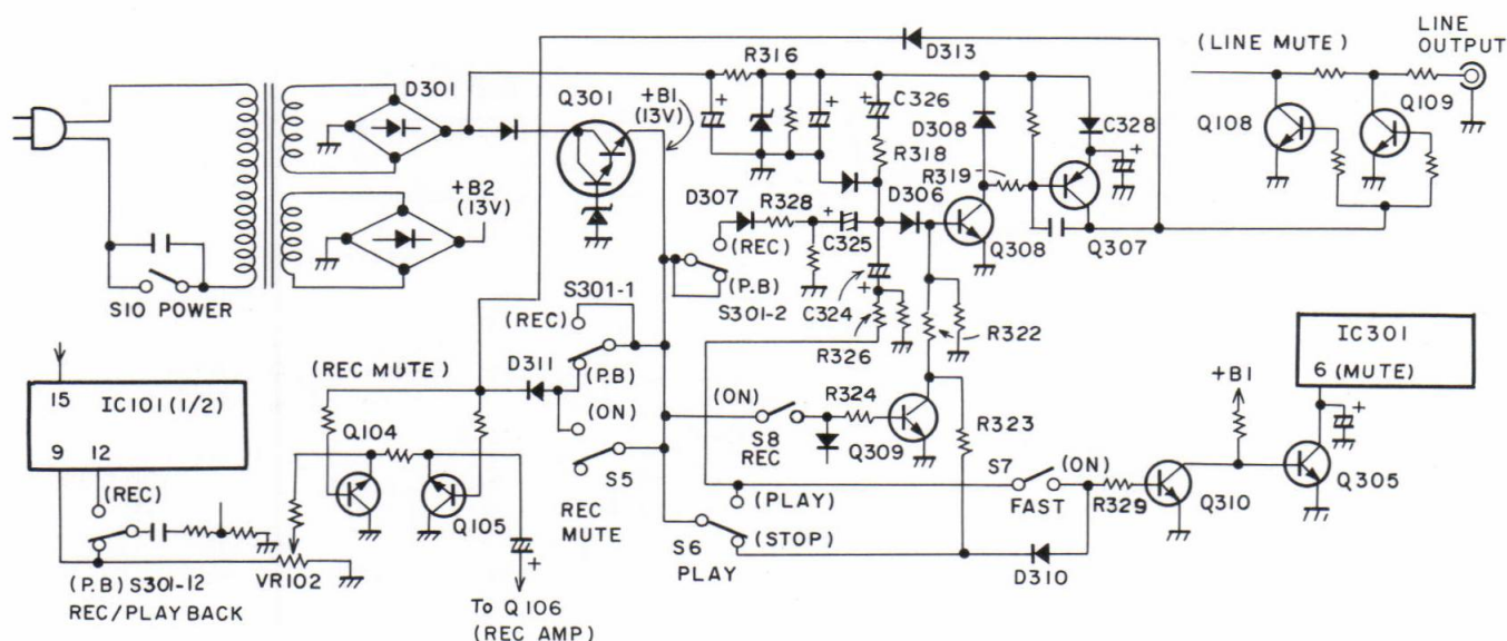
Fi. 6-1 Muting circuit
