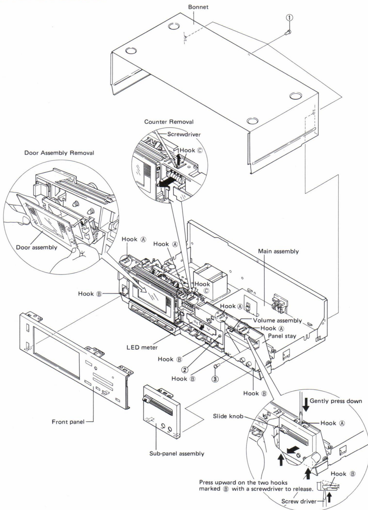
Fig. 3-1 Disassembly 1
