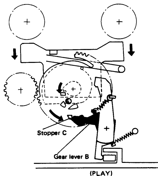
(PLAY) Fig. 2-10 PLAY → PAUSE operation 1
