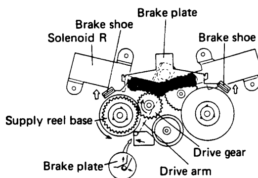
Fig. 1-15 Rewind operation
