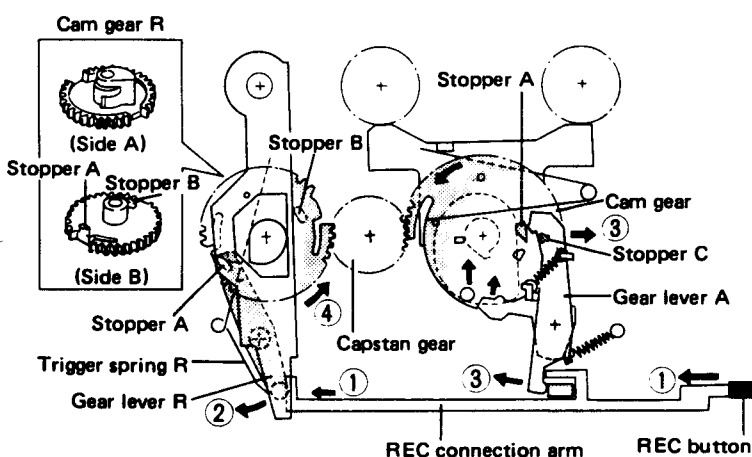
Fig. 2-12 STOP → REC operation
