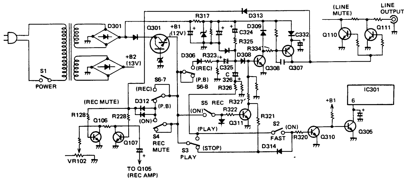
Fig. 2-1 Muting circuit
