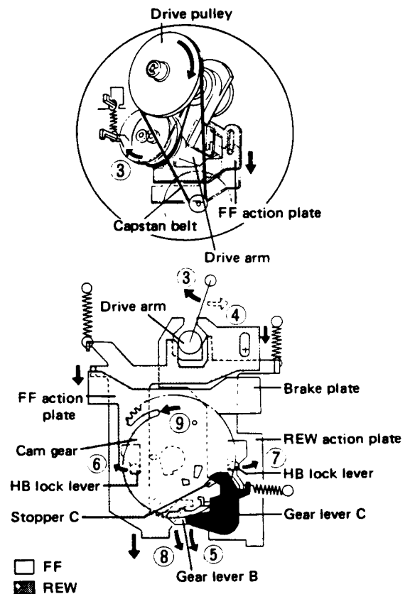
Fig. 2-17 FF (REW) operation
