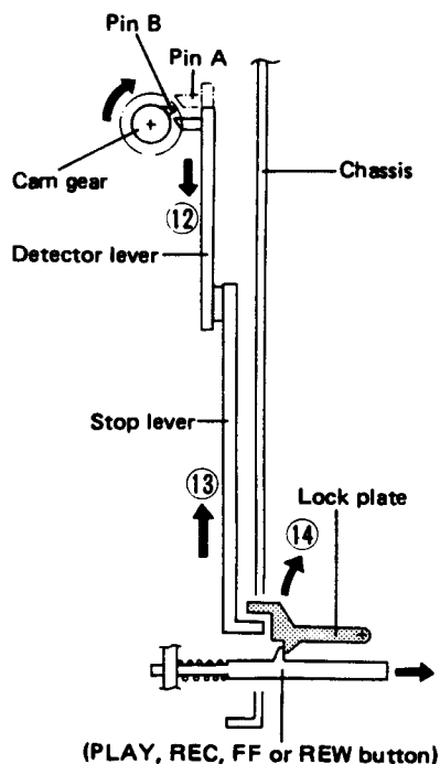
Fig. 2-20 Auto-stop operation
