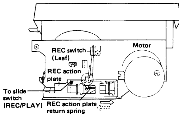
Fig. 2-14 STOP → REC operation (REC switch ON)
