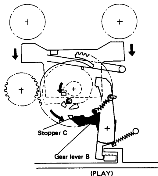
Fig. 2-10 PLAY → PAUSE operation 1
