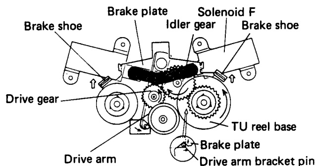
Fig. 1-14 Fast forward operation
