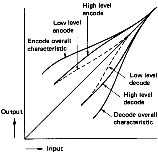
Fig. 1-3 Input/Output characteristic
