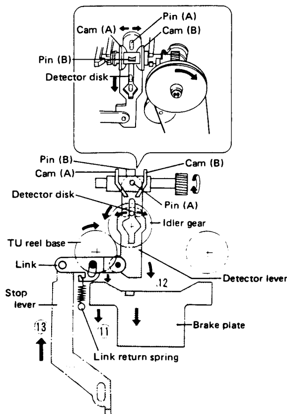
Fig. 2-19 Auto-stop operation
