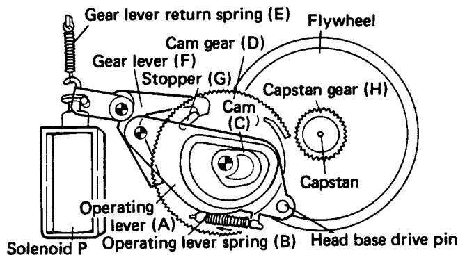
Fig. 1-8 STOP operation
