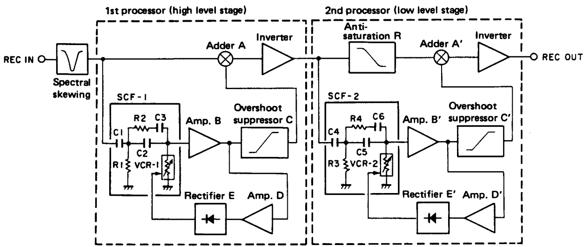
Fig. 1-1 Block diagram for encoding operation
