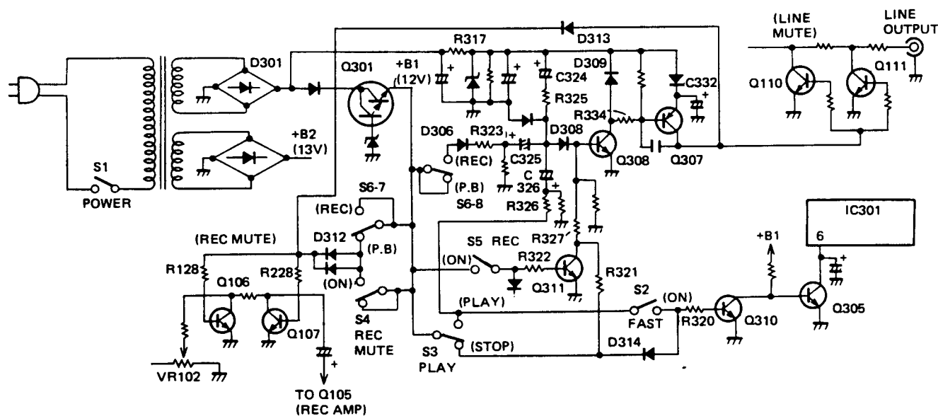
Fig. 2-1 Muting circuit
