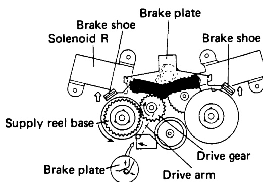
Fig. 1-15 Rewind operation
