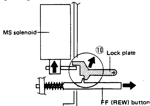
Fig. 2-18 FF (REW) button release
