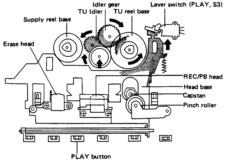
Fig. 2-7 PLAY operation
