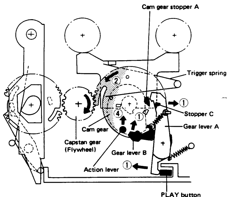
Fig. 2-5 STOP → PLAY operation
