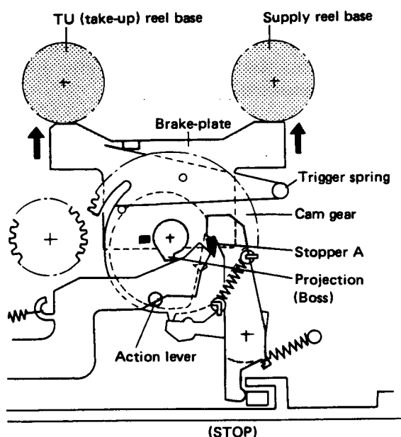
Fig. 2-9 PLAY → STOP operation
