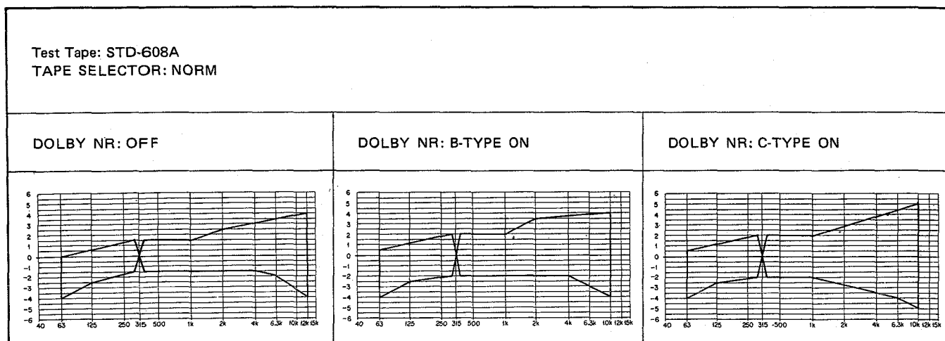
Fig. 10-8-1 Allowable recording and playback frequency response zone (NORM)
