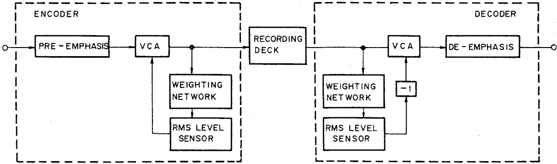
Fig. 1-2 dbx System block diagram
