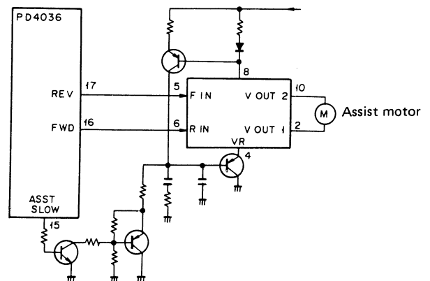
Fig. 4-8 Assist motor drive circuit
