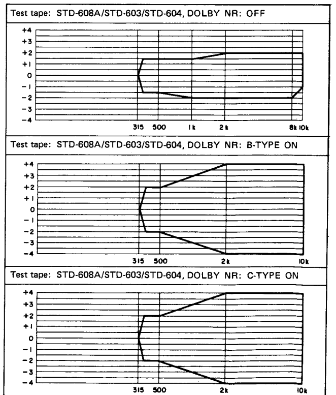
Fig. 11-13 Allowable recording/playback frequency response zone (NORM, AUTO-BLE)
