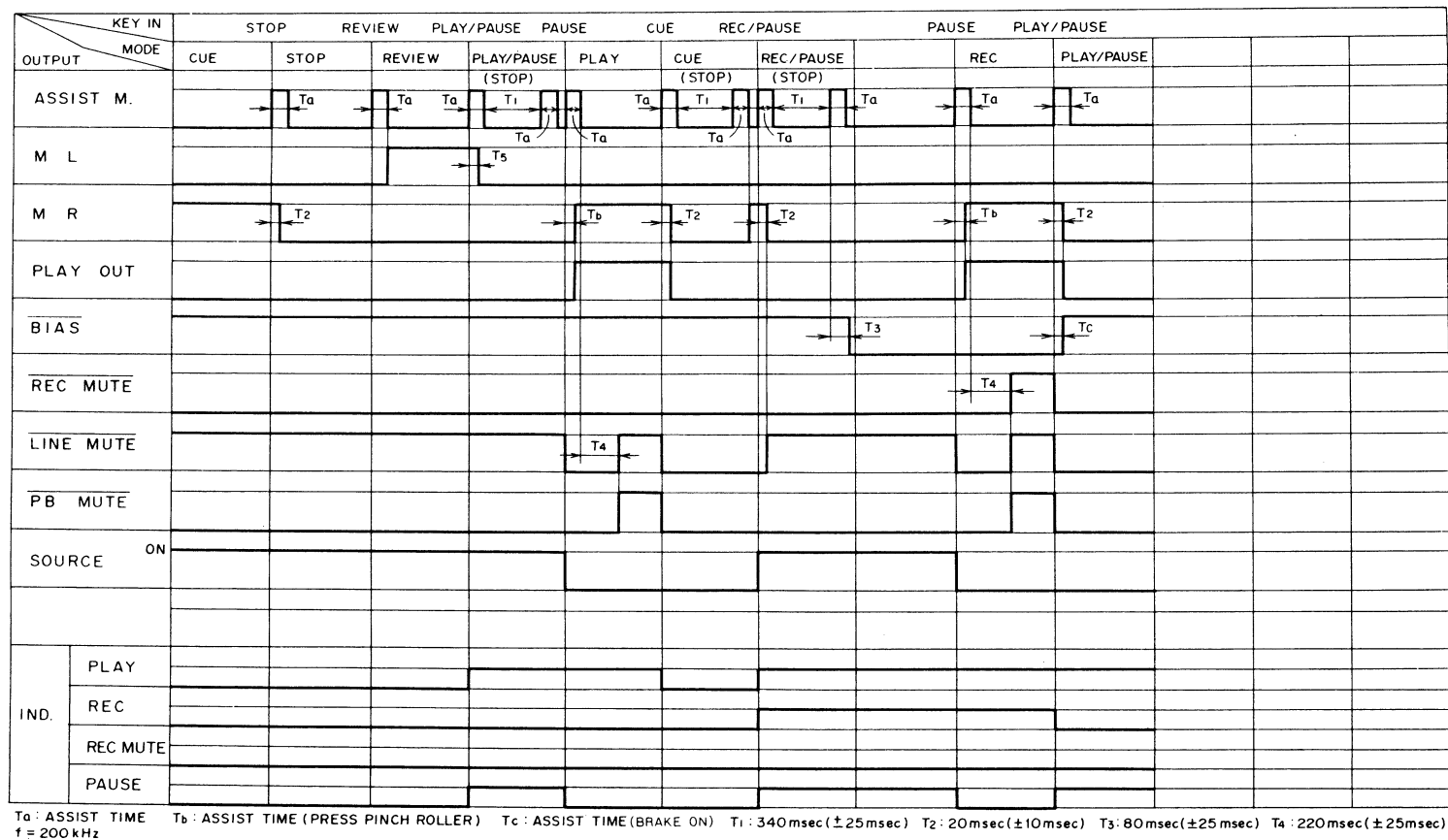
Fig. 4-36 Timing chart 7
