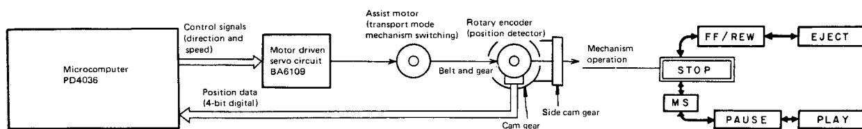
Fig. 1-1 Assist motor control circuit
