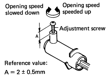
Fig. 11-2 Air damper adjustment
