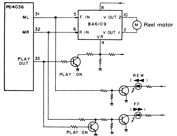
Fig. 4-7 Reel motor drive circuit
