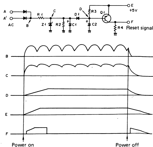
Fig. 4-5 Reset circuit
