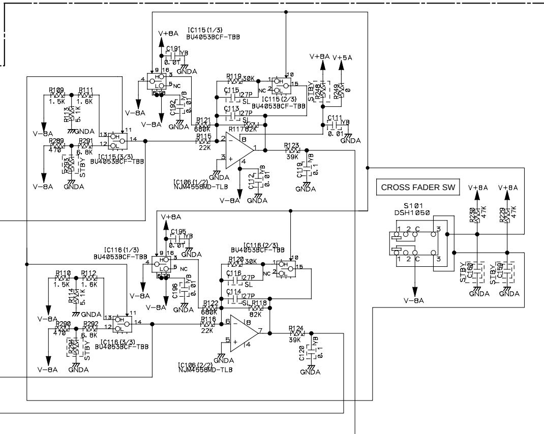
D 6/6 VR ASSY (6/6) (DWG1517)
