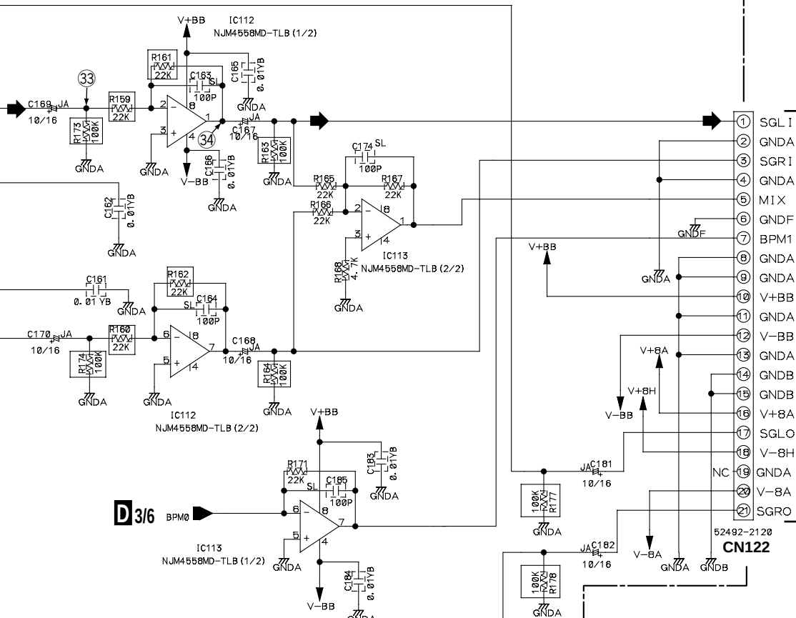
D 6/6 VR ASSY (6/6) (DWG1517)
