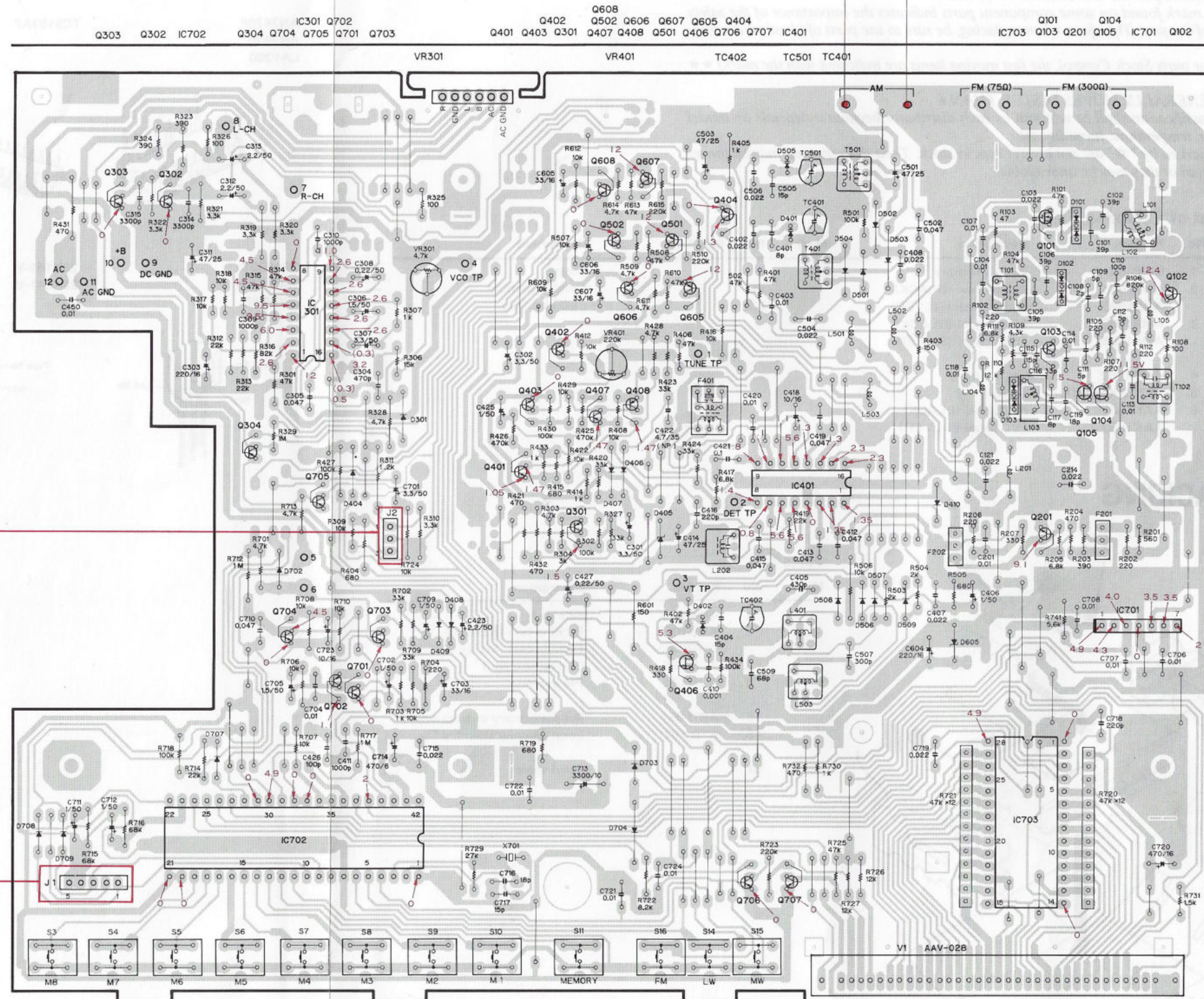
TUNER ASSEMBLY(GWE-270)
