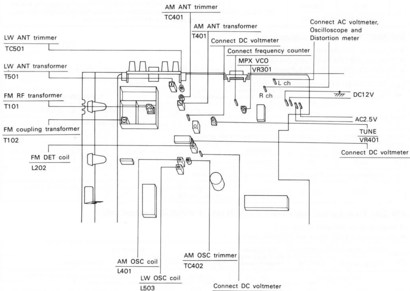
Fig. 12-3 Adjustment positions
