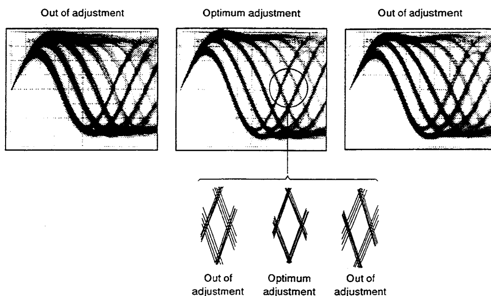
Figure 3 Eye pattern
