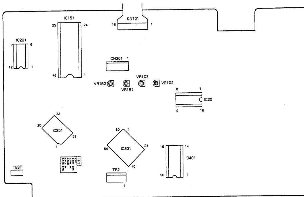
Figure 1 Adjustment Locations
