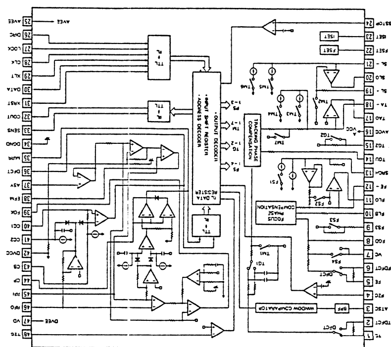
IC151: CXA1372S
