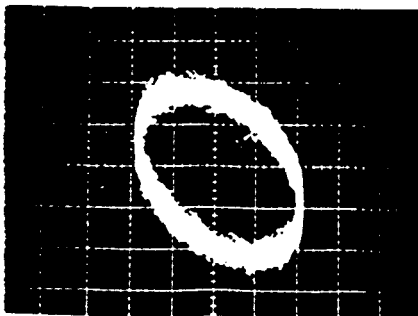
Gain overcompensated Photo 9-10
