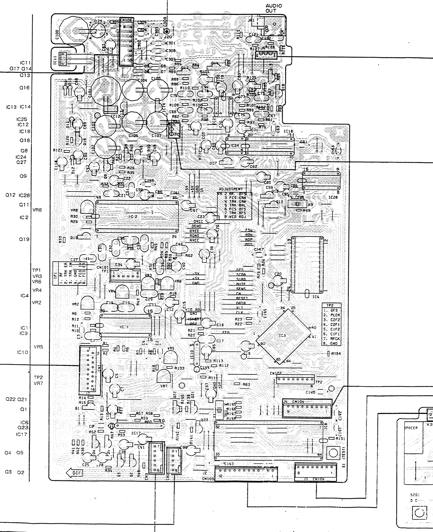
HEADPHONE BOARD ASSEMBLY
