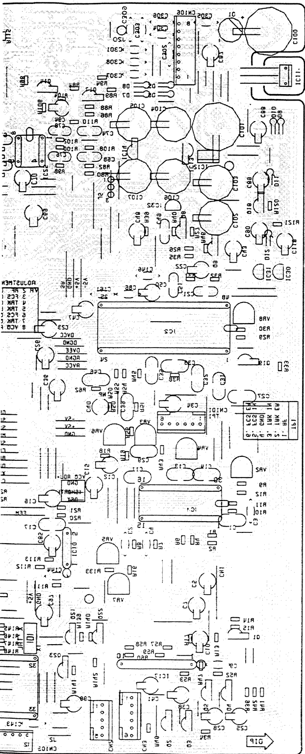
MAIN BOARD ASSEMBLY (PW51451)
