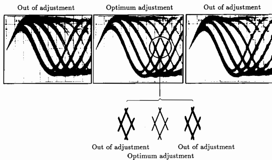
Figure 5 Eye pattern
