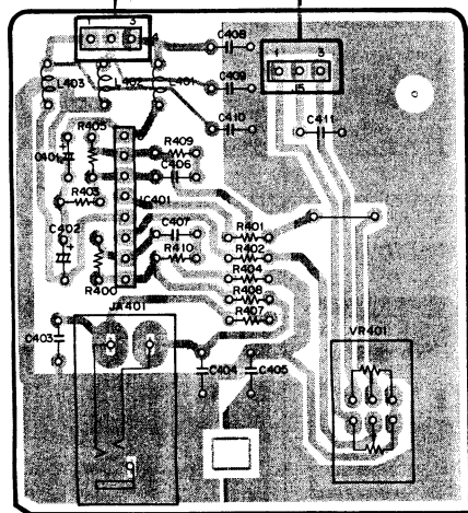
HEADPHONE ASSEMBLY
