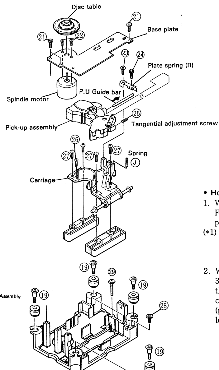
Fig 3-3 Parts disassembly (Servo mechanism assembly)
