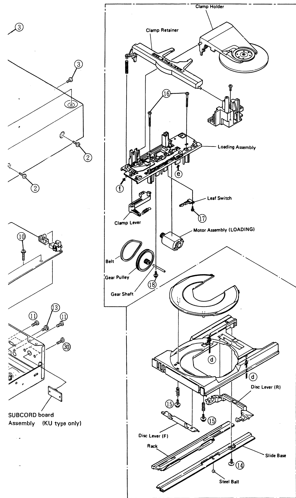
Fig 3-2 Parts disassembly (Loading mechanism and Tray assembly section)
