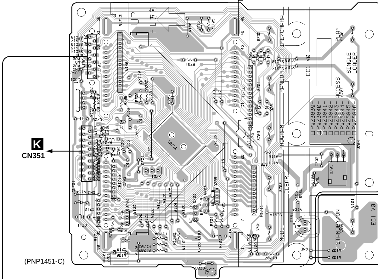
M FUNCTION BOARD ASSY
