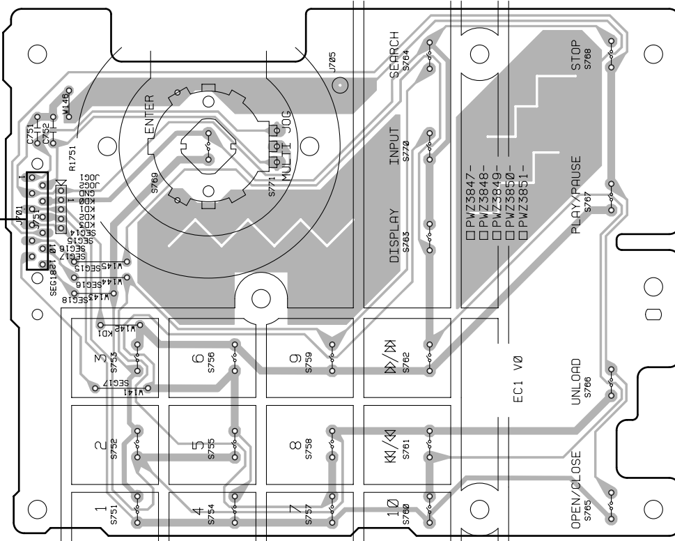
M FUNCTION BOARD ASSY
