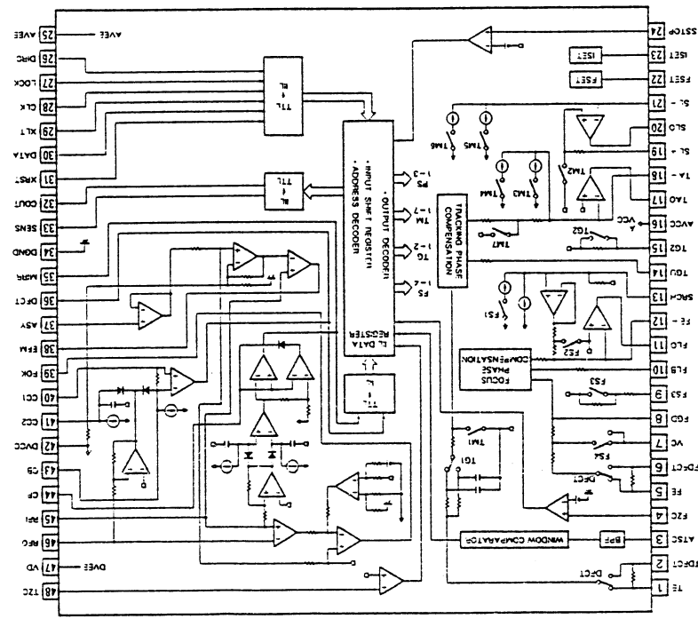
IC151: CXA1372Q
