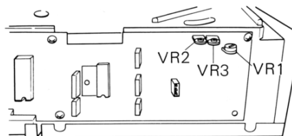
Fig. 9.3 End Detector Adjustment 2
