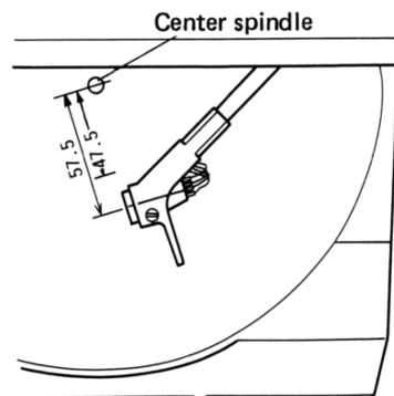
Fig. 9.2 End Detector Adjustment 1
