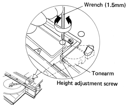
Fig. 9.6 Stylus Height Adjustment
