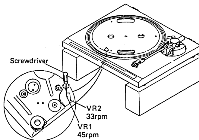
Fig. 11-3 Motor adjustment
