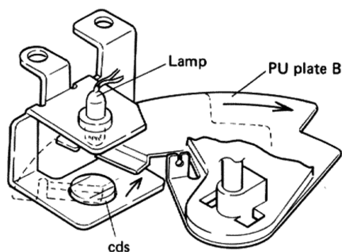
Fig. 10 End detector sensor
