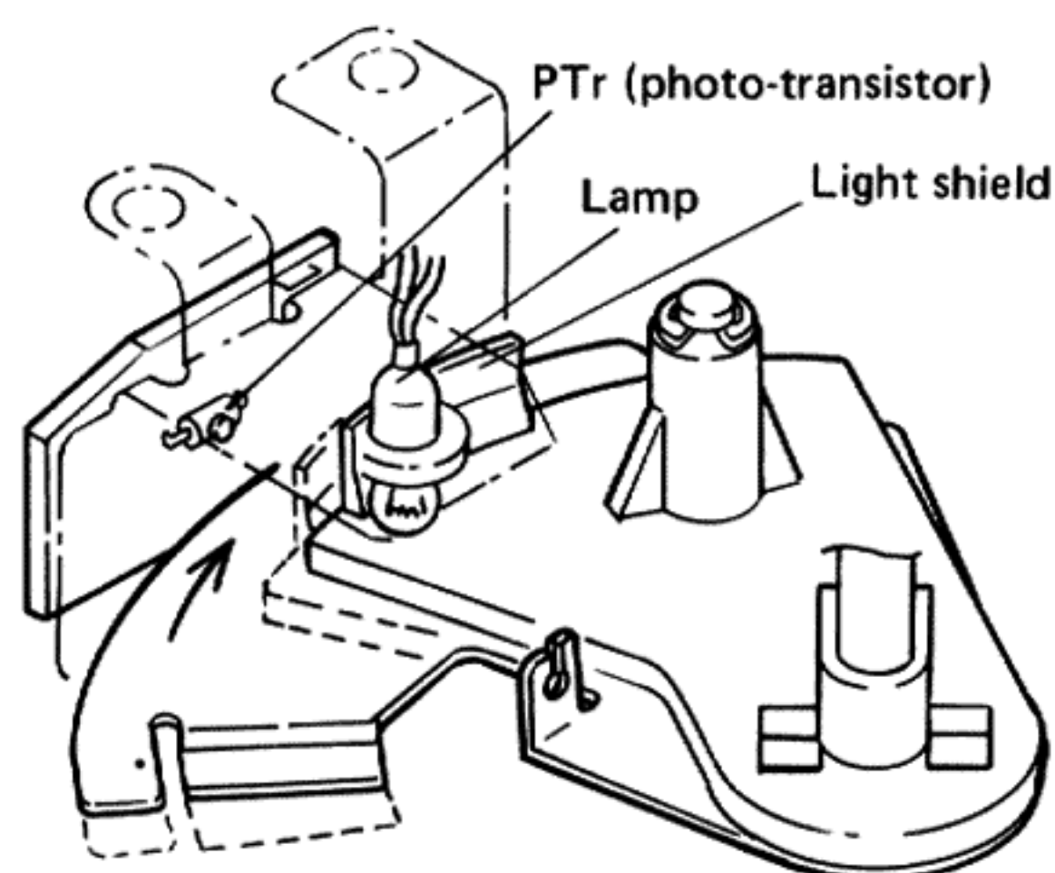
Fig. 11 Rest switch
