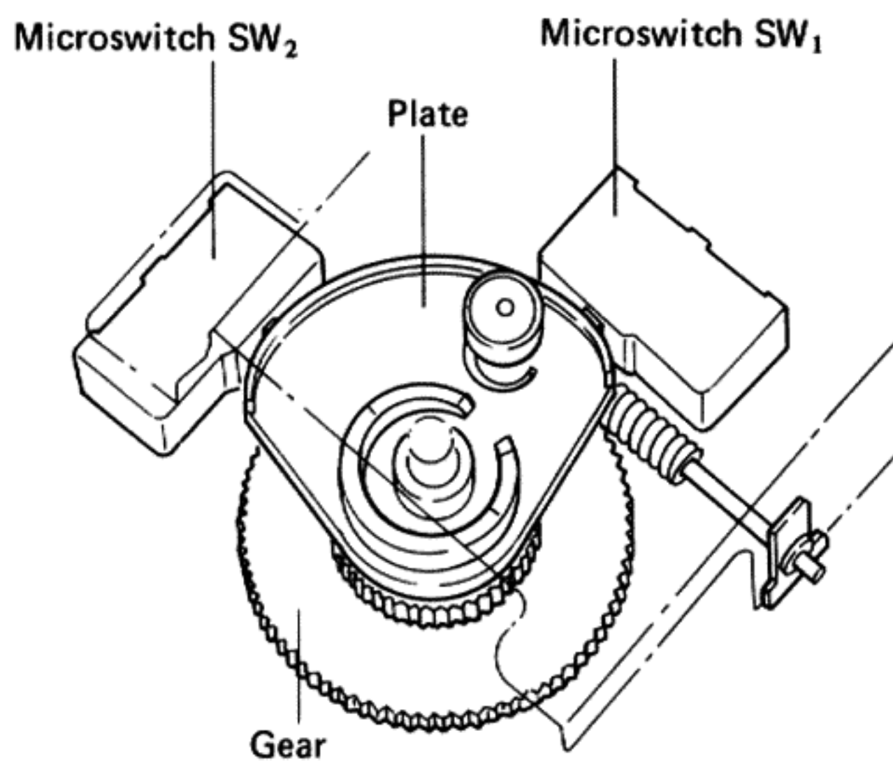
Fig. 5 Neutral position
