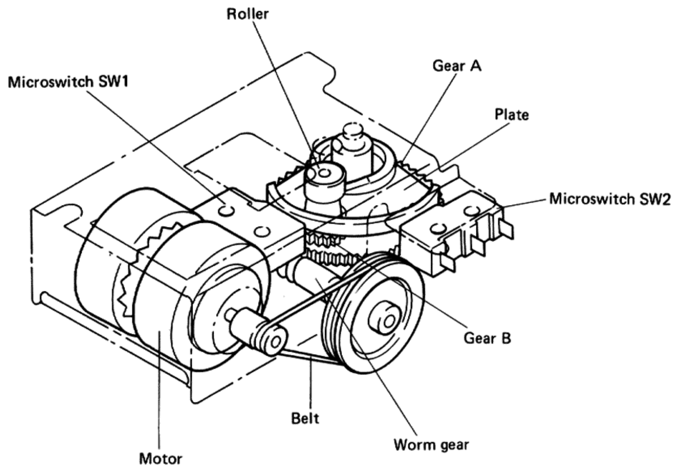
Fig. 4 Construction
