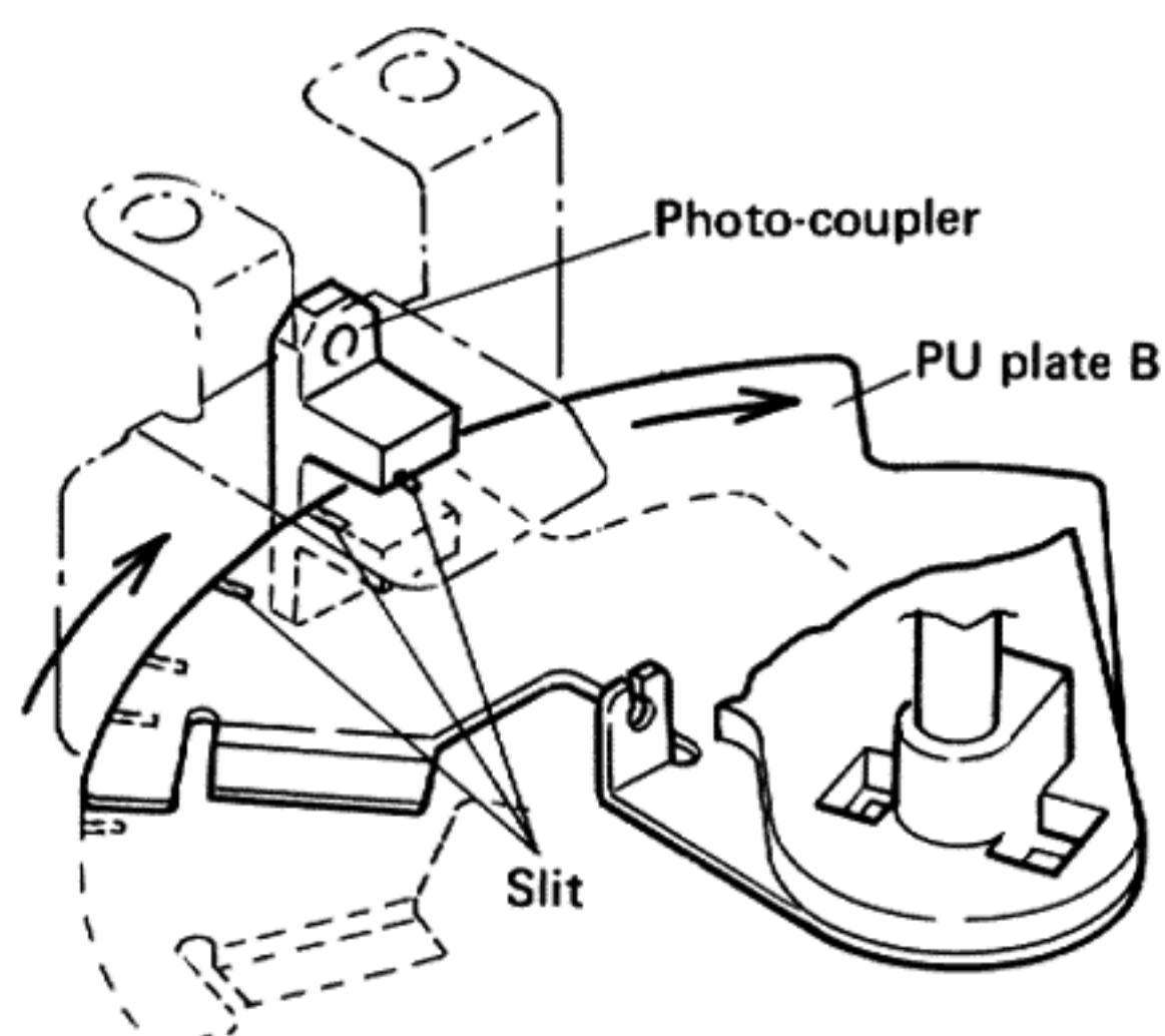
Fig. 9 Lowering position sensor
