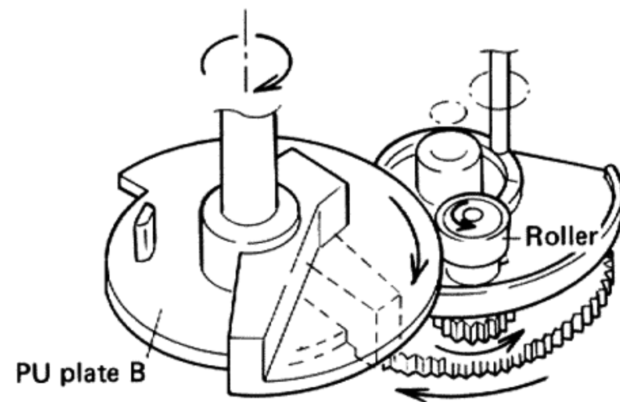
Fig. 7 Tonearm lead in
